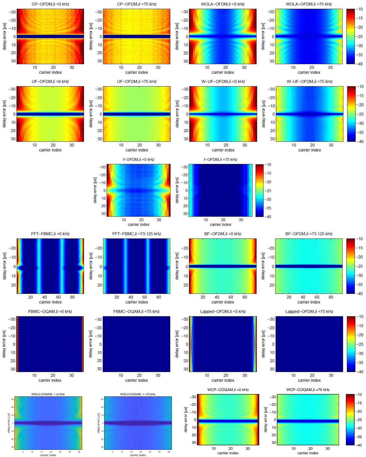
Figure 4.5: Per-subcarrier NMSE against TO.
