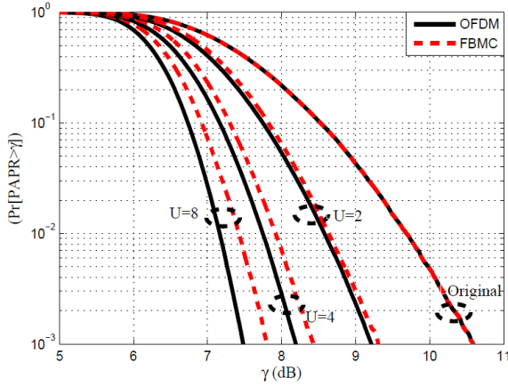
Figure 5.10: CCDF of PAPR comparison of DSLM and classical SLM schemes in FBMC-OQAM with N = 64 and U = [2, 4, 8] .
