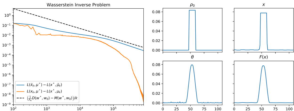
Figure 5.5: (Left) Ergodic and pointwise convergence profiles for Algorithm 10 applied to the Wasserstein inverse problem with entropic regularization parameter \gamma = 1 , total variation regularization parameter \beta = 1 , and n = 108 . (Right) The ground truth measure \rho_0 , the recovered measure x , the corrupted observation \theta , and the image of the recovered measure F(x) .
