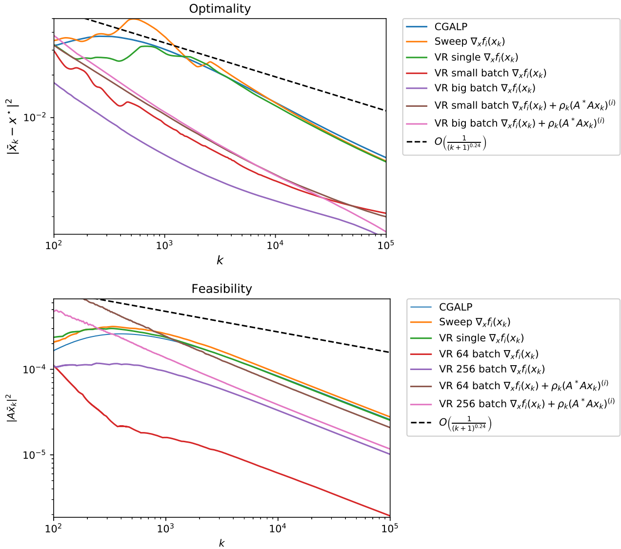
Figure 4.1: Ergodic convergence profiles for ICGALP applied to the projection problem (4.5.1) with n = 1024 . The step size is, for each k \in \mathbb{N} , \gamma_k = (k+1)^{-(1-\frac{1}{4}+0.01)} and the weight for variance reduction is, for each k \in \mathbb{N} , \nu_k = \gamma_k^{\frac{2}{3}} .
