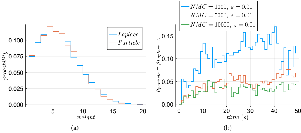
Figure 3.3: (3.3a) In blue: distribution of the process (\overline{W}_t)_{t \geq 0} at time t = 3s obtained from 10^4 trajectories simulated using the Laplace transform. In red: distribution of the process (W_t^\varepsilon)_{t \geq 0} at time t = 3s obtained from 10^4 trajectories of the process (V_t^\varepsilon, S_t^\varepsilon, W_t^\varepsilon)_{t \geq 0} . (3.3b) Distance in norm L_1 between the two distributions through time. Parameters are the same as Figure 3.2 with \beta = \alpha_M = 1 \text{ ms}^{-1} , \alpha_m = 0.05 \text{ ms}^{-1} and \varepsilon = 0.01 .
