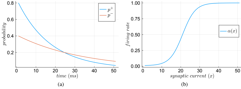
Figure 3.2: (3.2a): Functions p^+(\cdot, \hat{w}) and p^-(\cdot, \hat{w}) with parameters A_+=0.8 , A_-=0.4 , \tau_-=2\tau_+=34 ms. (3.2b): Sigmoid function \alpha with parameters \alpha_m = 0.01 \text{ ms}^{-1} , \alpha_M = 1 \text{ ms}^{-1} , \sigma = 0.3 , \theta = 20 .
