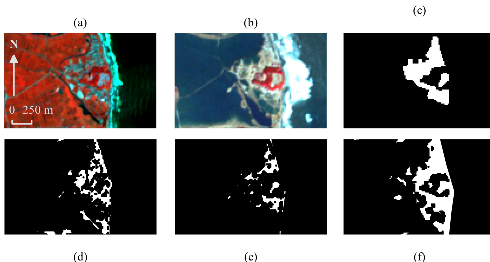
Figure 2.13: Clustering results, destroyed constructions. (a) image taken on 7 July 2010, (b) image taken on 19 March 2011, (c) ground truth, (d) K-Means on subtracted image, (e) K-Means on concatenated encoded images, (f) DEC on concatenated encoded images.
