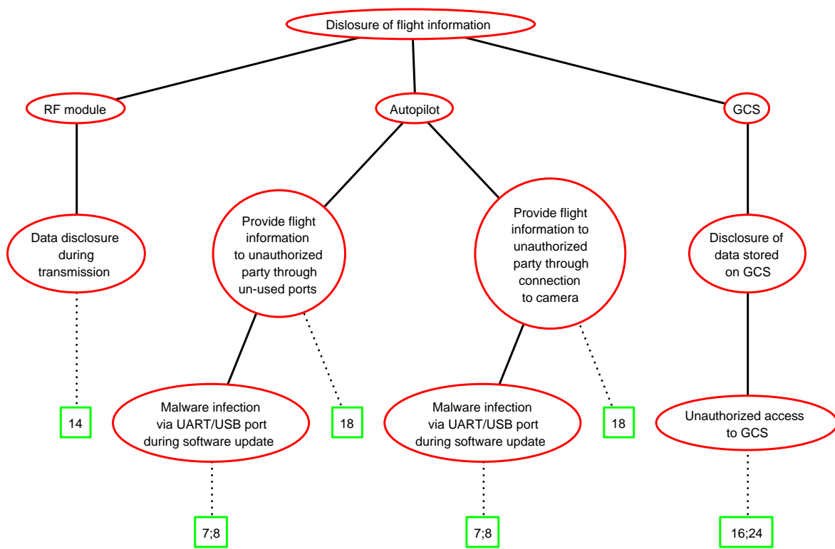
Figure C.7: The attack tree for the 2-confidentiality malfunction
