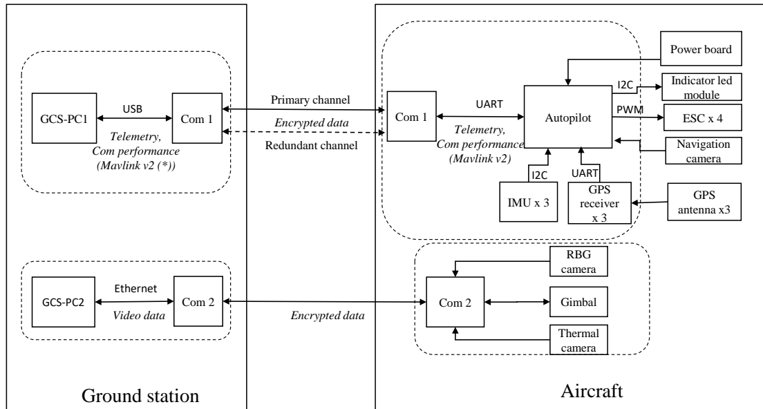
Figure 5.5: System Architecture
