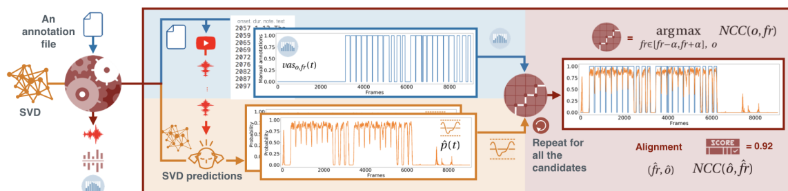
Figure 4.6: The input is an vas_{o,fr}(t) (blue part) and a set of audio candidates retrieved from Youtube. The similarity estimation method uses a SVD model (orange part) to convert each candidate in a \hat{p}(t) (orange part). We measure the similarity between the vas_{o,fr}(t) and each \hat{p}(t) using the cross-correlation method \arg \max_{fr,o} NCC(o, fr) (garnet part). The output is the audio file with the highest NCC(\hat{o}, \hat{fr}) and the annotations aligned to it using \hat{fr} and \hat{o} .
