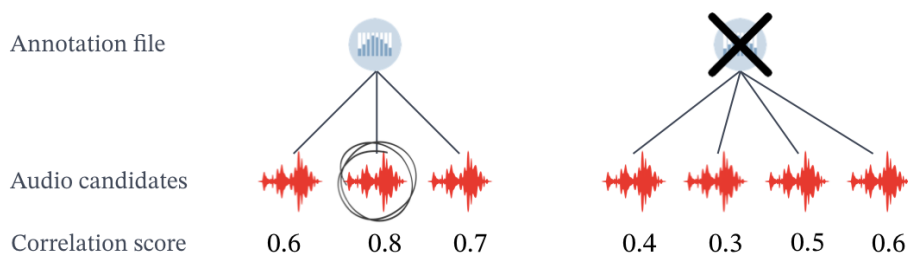
Figure 4.5: In order to discover its best alignment for each candidate, annotations are modified by changing its offset_time and frame_rate . The candidate with the highest NCC value is our final audio track. This similarity is not only important in recovering the correct audio and finding the best alignment but also in determining if annotations are accurate enough. Fixing a threshold we can filter imprecise annotations.
