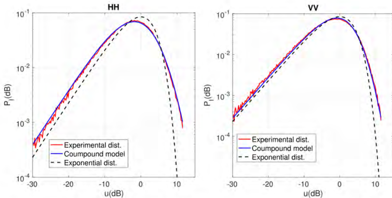
Fig. 12. Normalized intensity distribution (in logarithmic scale) from (7) according to the compound distribution model with corrected PR ( \alpha = 0.6 ) at 45^\circ incidence with mss_r = 0.0113 for the horizontal (HH, left panel) and vertical (VV, right panel) polarization. An excellent agreement with the POLLUPROOF experimental data is obtained simultaneously for the two copolarization states with the same value of mss_r . The exponential distribution is given for reference.
