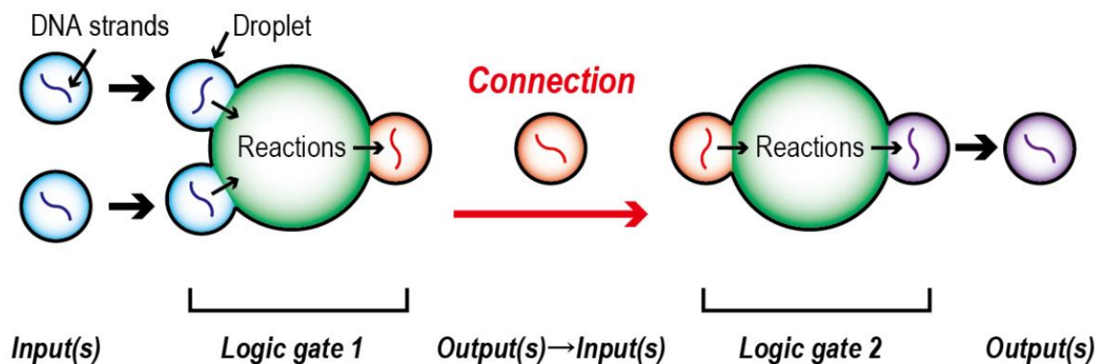
Figure 1.20. Elaboration DNA logic gates in droplets.
