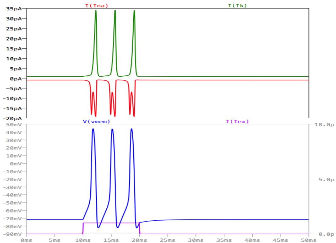
Figure 3.8 Response of the biomimetic neuron with 8 transistors to a pulsed current. With I_{ex} = 1\text{pA} and T_s = 10\text{ms} . I(Ik) corresponds to the potassium current (IK) and I(Ina) corresponds to the sodium current (INa). The action potential is in blue V(vmem) and the excitatory current I(Iex) is in pink.
