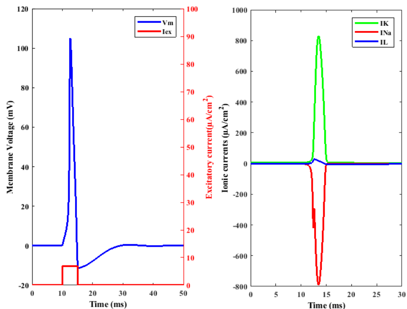
Figure 2.11 Generation of one spike with HH model. Left: Membrane voltage for a pulsed excitatory current with I_{ex} = 7 \mu A/cm^2 and T_s = 5ms . Right: Ionics currents, I_{Na} , I_K and I_L .
