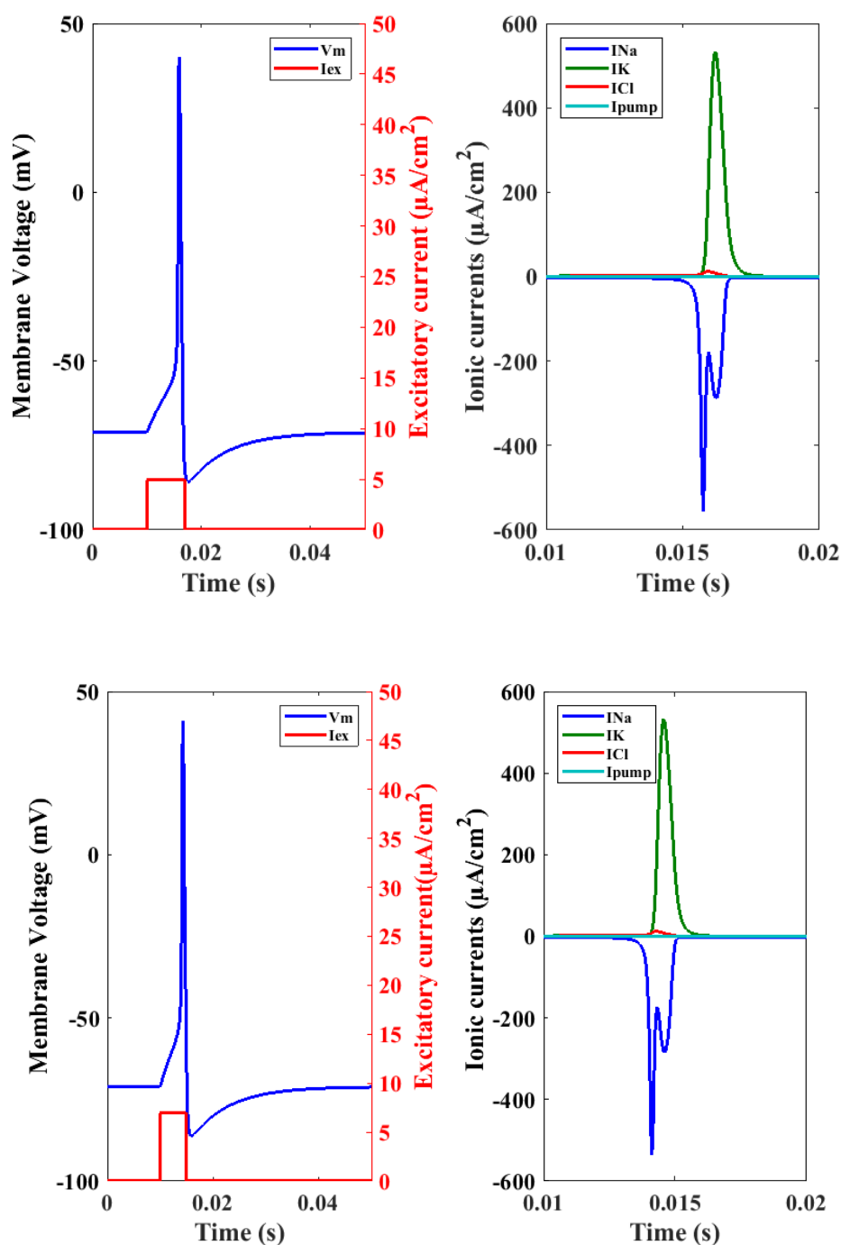
Figure 2.17 Generation of one spike with Wei model. Figure.2.17.up: V_m is generated for I_{ex} = 5 \mu\text{A}/\text{cm}^2 and T_s = 7 \text{ms} . Figure.2.17.down: V_m is generated for I_{ex} = 7 \mu\text{A}/\text{cm}^2 and T_s = 5 \text{ms} .
