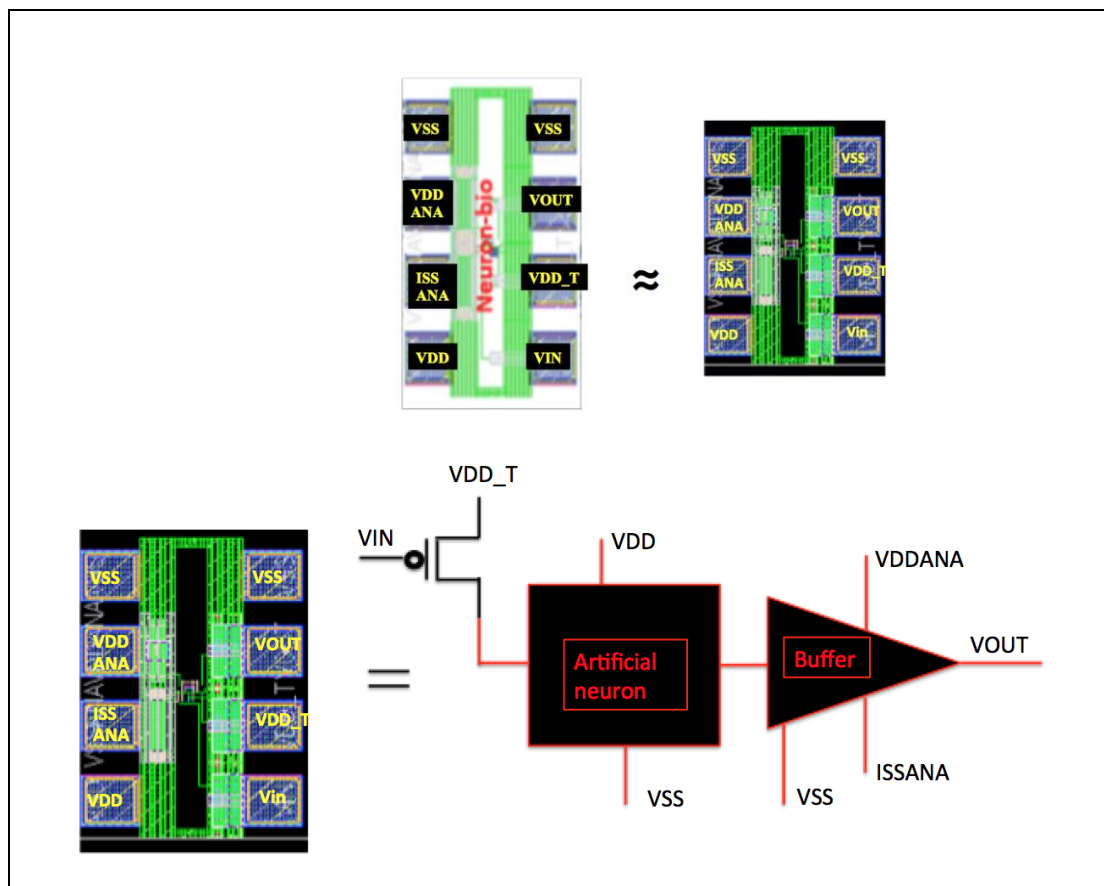
Figure 4.2 Artificial neurons circuits and schematic.
