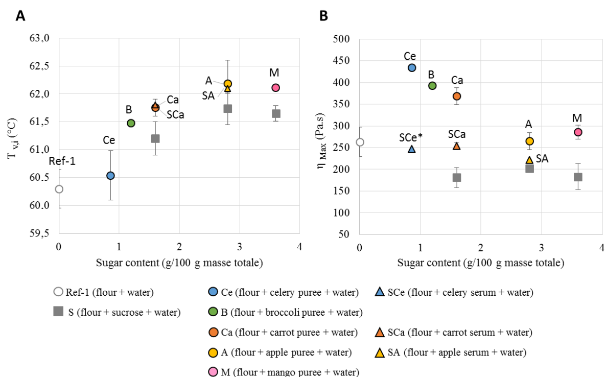
Fig. 15: Temperature from which the viscosity increased, T_{v,i} , and maximal viscosity during the temperature ramp, \eta_{Max} as function of sugar content for mixtures with 20 wt% of puree or serum and the corresponding wheat flour + water + sucrose mixtures. (*)Data were produced in triplicate except for the experiment with celery serum (one trial).
