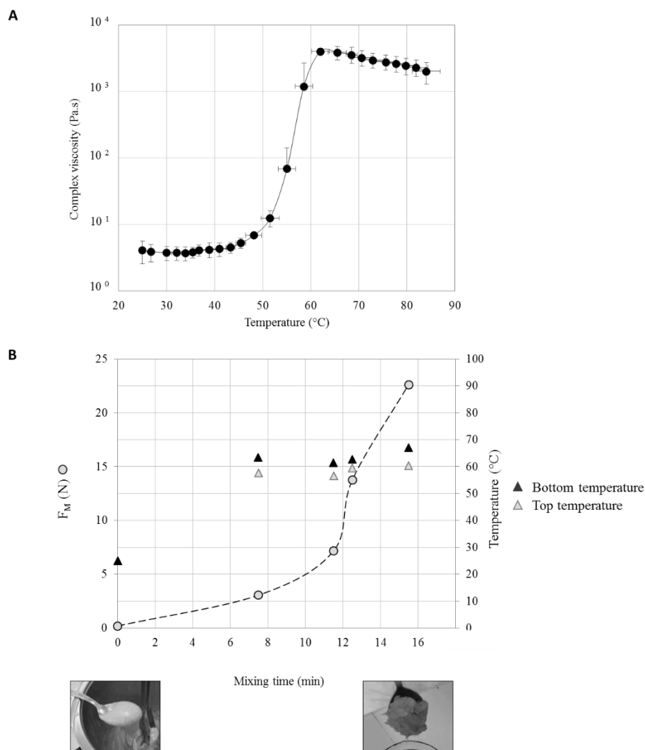
Fig. 8 : Increase of complex viscosity and normal resistance force ( F_M ) of dough at 65 wt% of water upon heating. (A) Complex viscosity at 1Hz (heating rate: 5 ^{\circ}\text{C}/\text{min} ; 0.2% strain); (B) F_M (after cooling) and temperature levels at different mixing times.
