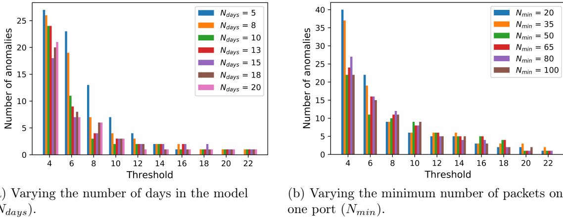
Figure 3.10: Number of anomalies depending on a parameter for diverse thresholds (2016).
