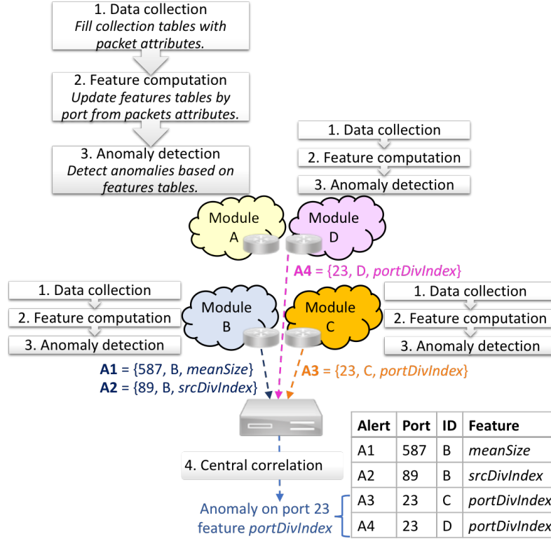
Figure 3.1: Architecture example. Local modules run at different points in the network and send alerts to the central correlation module. The controller will then be able to keep only distributed ones. Here it spots an anomaly on port 23 for feature portDivIndex , coming from two different places.
