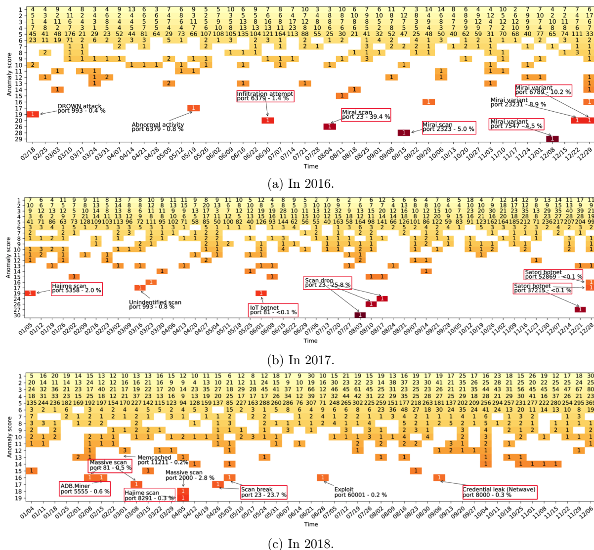
Figure 3.6: Anomaly scores for the MAWI dataset (number of anomalies for one port, taking into account all features and all monitors). In the coloured squares are given the numbers of ports with this anomaly score this day. Events detected in both datasets are tagged with a red frame.
