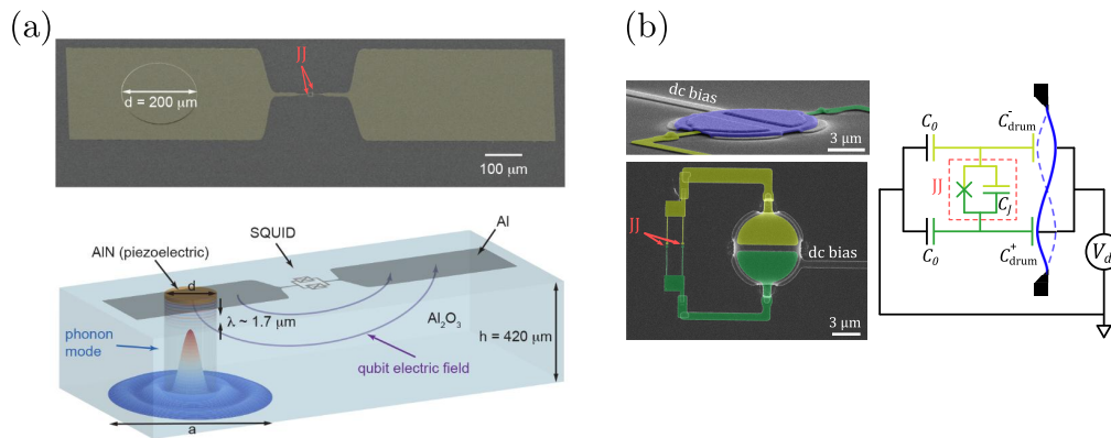
Figure 5.3: a , (Top) Optical micrograph of the top view of the BAR, on which the piezoelectric disk (diameter 200 \mu\text{m} ) and the Josephson Junctions (JJ) of the qubit can be seen. (Bottom) Schematic of the BAR resonator, indicating the localization of the phonon mode (not to scale) energy. Images extracted from Chu et al. [15]. b , (Top left) SEM image of the aluminium plate and the DB bias line. (Bottom left) SEM image of the aluminium plate and the charge qubit, seen from the top. (Right) Electric diagram of the electromechanical device, showing the aluminium plate (blue) and the Cooper-pair box (red box). Images extracted from [16].
