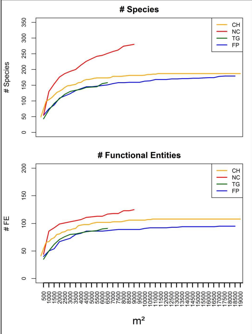
Figure S1. Accumulation curves for species and functional entities richness. Accumulation curves for species richness (top) and functional entities (bottom) for each of the four locations (Chagos, orange; New Caledonia, Red; Tonga, green; French Polynesia, blue) along transects (x-axis, m 2 ).
