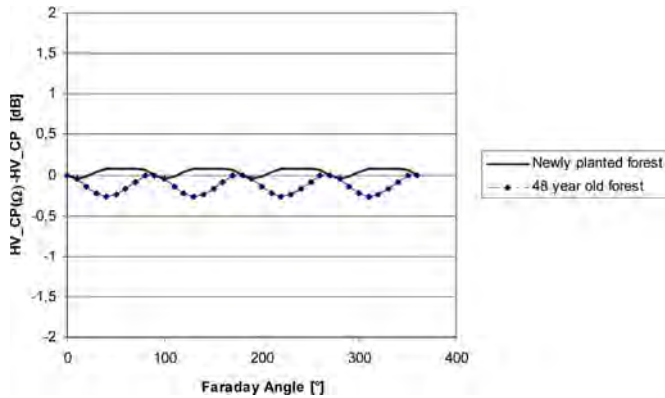
Fig. 3. Difference in the estimation of the HV backscattering coefficient from the CP mode in the presence of a Faraday rotation ranging from 0° to 360°. With this definition, the difference is null when there is no Faraday rotation.
