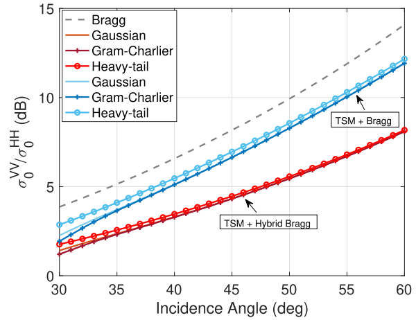
Fig. 7. X-band PR under the TSM and hybrid TSM ( \alpha = 0.6 ) obtained at 10 m/s wind speed with 1) different omnidirectional wave spectrum models and a Gaussian facet slope distribution (top panel) and 2) Elfofhaily omnidirectional wave spectrum and different types of isotropic facet slope distributions with equal mss: Gaussian, Gram-Charlier, or alpha-stable with parameter 1.7 (bottom panel). The pure Bragg PR is given for reference.
