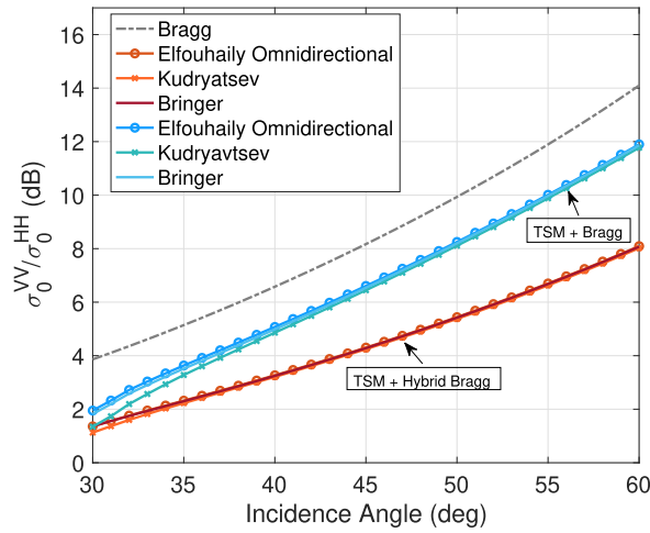
Fig. 7. X-band PR under the TSM and hybrid TSM ( \alpha = 0.6 ) obtained at 10 m/s wind speed with 1) different omnidirectional wave spectrum models and a Gaussian facet slope distribution (top panel) and 2) Elfofhaily omnidirectional wave spectrum and different types of isotropic facet slope distributions with equal mss: Gaussian, Gram-Charlier, or alpha-stable with parameter 1.7 (bottom panel). The pure Bragg PR is given for reference.
