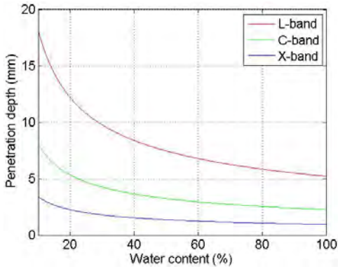
Fig. 1. Penetration depth as a function of water content (volumetric percentage) based on a linear mixing model for the dielectric constant at L-band (red), C-band (green), and X-band (blue); dielectric constants are specified in Table I.
