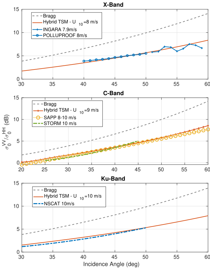
Fig. 8. Comparison of the modeled PR in the TSM+hybrid Bragg model with isotropic Elfofhaily spectrum and the measured omnidirectional NRCS in C-, X-, and Ku-bands for moderate wind speeds.
