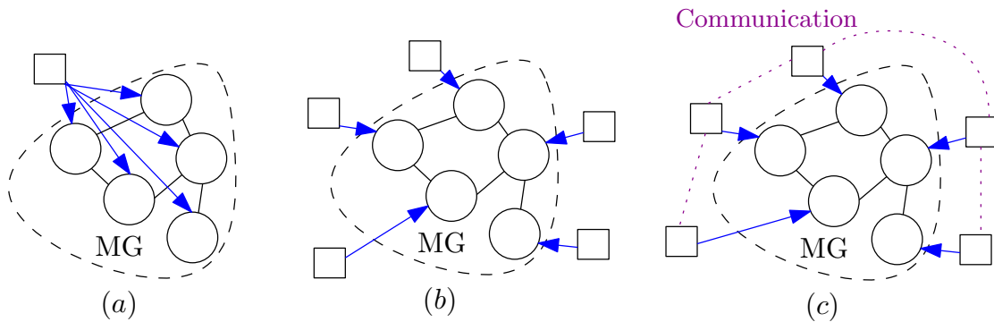
Figure 1.8: Illustration of the three main control architectures in MGs. From the left, centralized, decentralized and distributed control (o element of the MG and □ controller).
