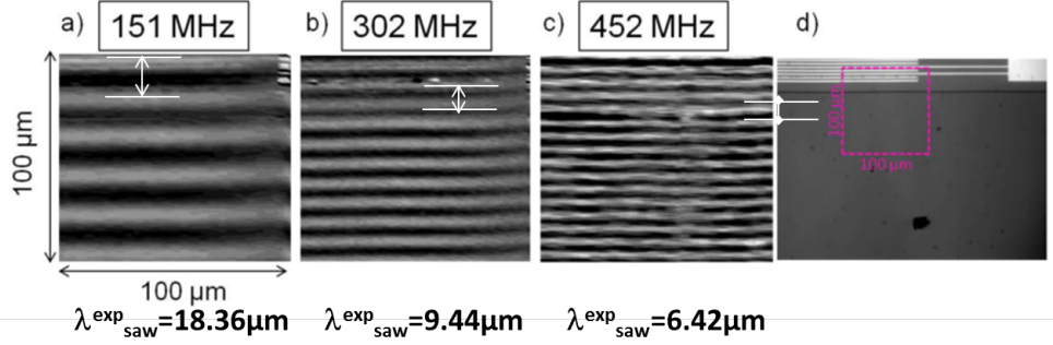
Figure IV.6: [110] Photoelastic effect maps of surface acoustic waves of frequency f_{saw} = n f_L ( n = 1, 2, 3 ) taken at room temperature on (Ga,Mn)As, at the edge of the IDT (last image: photo of the sample).
