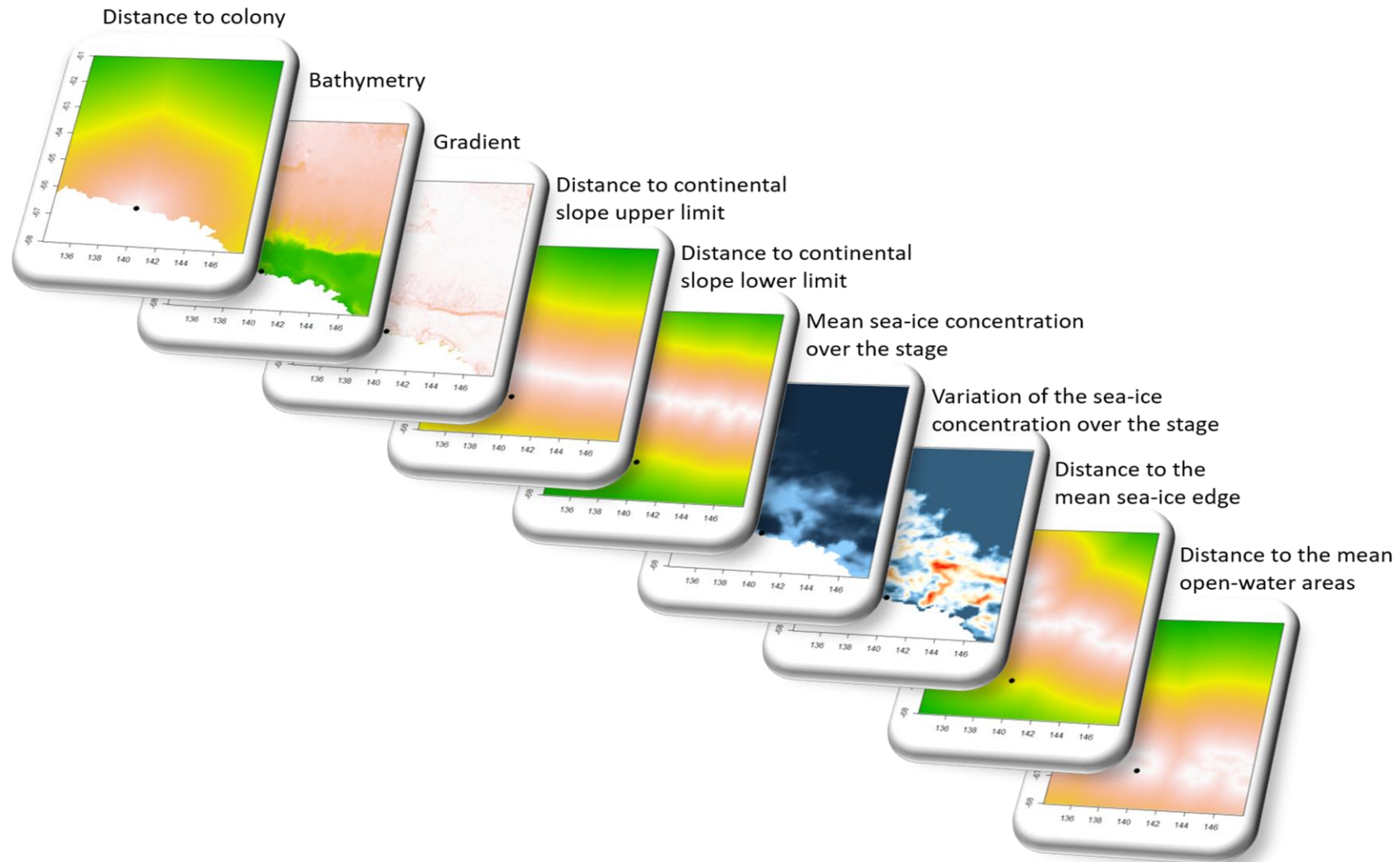
Figure S2: Summary of all environmental variables extracted and associated in each grid cell
