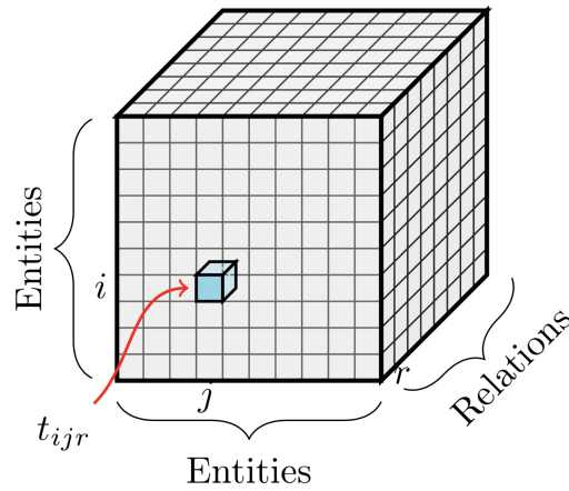
FIGURE 5.4 – Relational tensor.
