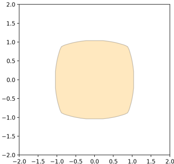
(f) Lovasz distance with f_4
