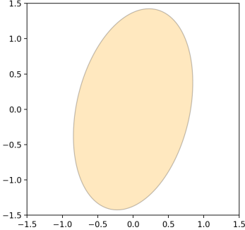
(b) Mahalanobis distance
