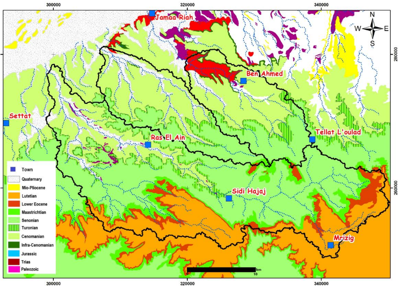
Figure 13: Geological and structural Map of Settât-Ben Ahmed plateau (adapted from El Gasmi et al. (2014b))
