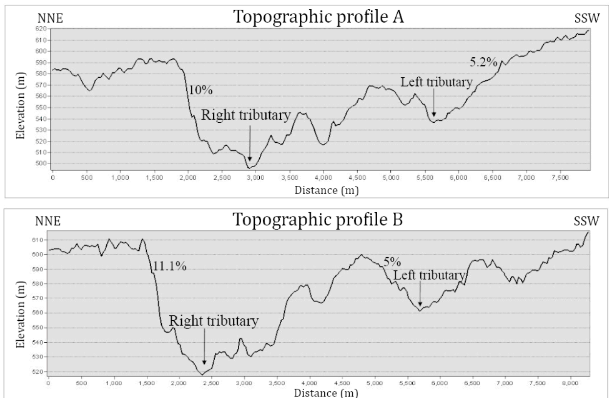
Figure 32: Topographic profiles of El Himer River
