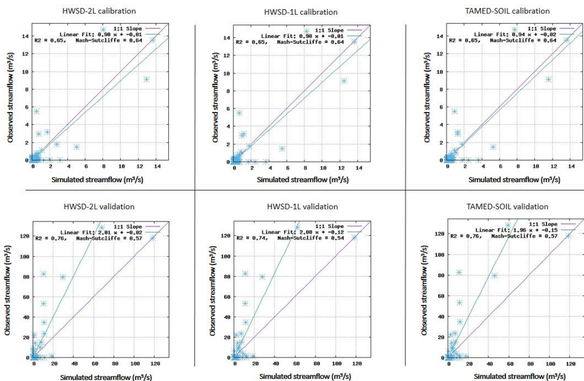
Figure 25: Scatter plot of simulated versus observed streamflow for the calibration (1998-2000) and the validation (2001-2002) periods for the three databases
