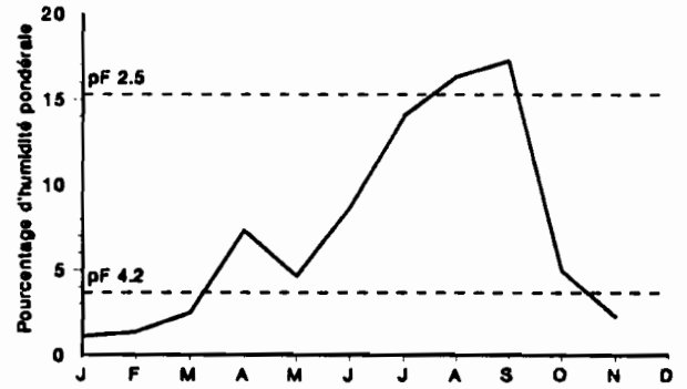
(5) SAVANE BOISEE A ISOBERLINIA DOKA -10 A -20 CM
