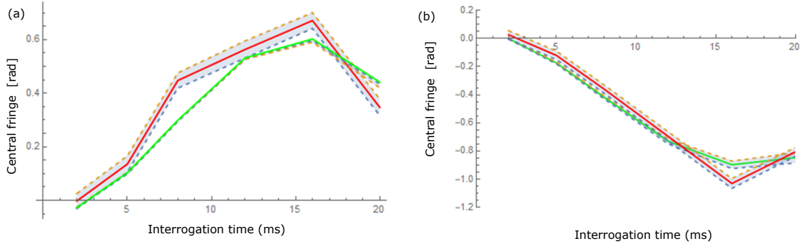
FIGURE 3.11 – Comparison of our model with the measurement of the central fringe for the Potassium interferometer. For each direction of the effective wave vector of the Raman beam ((a) +k_j and (b) -k_j ), estimated central fringe (green) based on the systematic errors study (Quadratic Zeeman effect, one photon and two photon light shift) and measured central fringe (red) versus the interrogation time. The margin for our model are defined by changing the initial velocity of the cloud by \pm 0.1v_R . The uncertainty on the measured fringes comes from the residuals of the fit.
