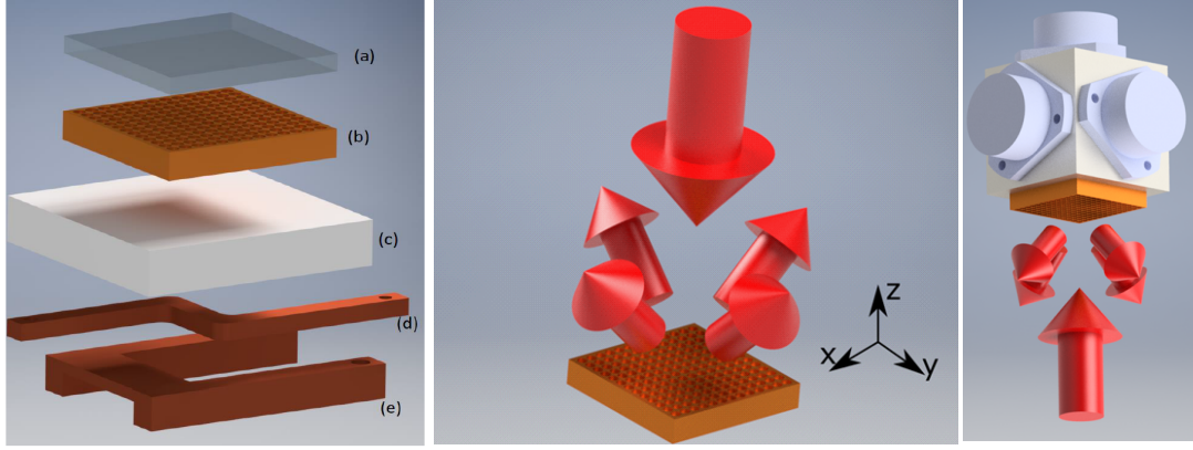
FIGURE 4.23 – (left) We envision to combine several techniques and configurations to create the ideal chip for multi-axis atom interferometry. This chip would include wires on a printed circuit board to generate the magnetic field(d)-(e), the optical grating (b) and a dichroic coating (a). (middle) The incoming and diffracted beams overlap above the grating where the MOT and optical molasses are realized. The same beams will be used as pairs of Raman beams. (right) The atom interferometers will be subsequently hybridized with classical accelerometers to form a low-bias, high-dynamic range, high-bandwidth inertial sensor.
