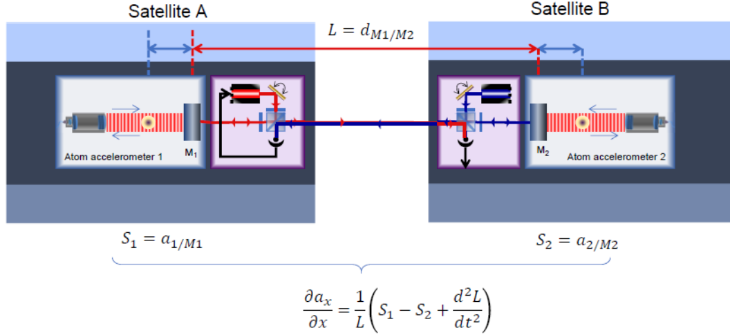
FIGURE 4.21 – Mission scenario involving twin satellites each equipped with a cold atom accelerometer. A laser telemeter is used to monitor the distance between the two satellites and couples the measurements of the two atom interferometers.
