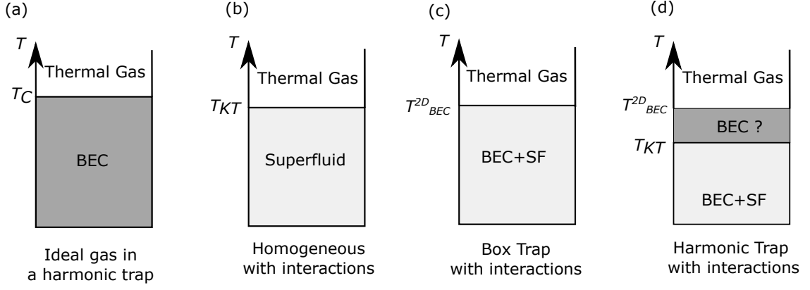
FIGURE 5.1 – Different existing phases in a 2D Bose gas. (a) In the case of a ideal gas localized in an harmonic trap, there is a non-zero critical temperature T_c under which there is a Bose Einstein condensate (BEC). (b) In the case of an homogeneous gas with interactions, there is no true condensate at non-zero temperature but there is a superfluid phase corresponding to a quasi-condensate with a fluctuating phase below a critical temperature T_{KT} . In the case of a gas with interactions localized in a box trap, the situation is complex and two different regimes are possible depending on the size of the system. For large systems, the situation tend towards the case (b) of the infinite homogeneous gas, and the BEC transition is BKT-driven (or in other words interactions-enhanced). (c) For small systems, There is a standard BEC transition first as in the case of the ideal gas. (d) In the case of the harmonic trap, the situation depends of the experimental parameters.
