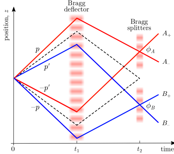
FIGURE 5.8 – Schematic diagram of the protocol used to observe two particle interference (LCF). An atomic four wave mixing effect creates a pair in a superposition : |p, -p\rangle + |p', -p'\rangle . Laser standing waves then act as deflectors and beam splitters to mix the different momentum modes. Interference is detected in the correlations between detectors at the A and B outputs. High enough fringe contrast can lead to the violation of a Bell inequality.
