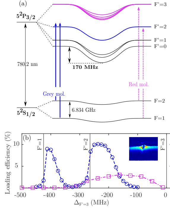
FIGURE 2.14 – (a) Level structure of the atoms including the light shift due to the painted ODT ( P \simeq 10 W, h = 100 \mu\text{m} ). The cooling and repumping frequencies are shown for the grey (solid blue lines) and red (dashed pink lines) molasses. The cooling and repumping light intensities are respectfully I_{\text{cool}} \approx 6I_S and I_{\text{rep}} \approx 0.6I_S . The light shift of the excited (ground) state at the center of the ODT is \sim 170 MHz (2.5 MHz). (b) ODT loading efficiency as a function of the detuning relative to |F = 2\rangle \rightarrow |F' = 3\rangle for the red (pink squares) and grey (blue circles) molasses. The atom numbers are estimated from absorption imaging. For each point, 5 images have been taken, averaged and fitted with a 2D gaussian profile. The standard deviation of the fit residuals gives an uncertainty of 5% about the loading efficiency. Inset : absorption image of atoms in the ODT using near-resonant light. Atoms at the center of the trap are transparent to the cooling beams.
