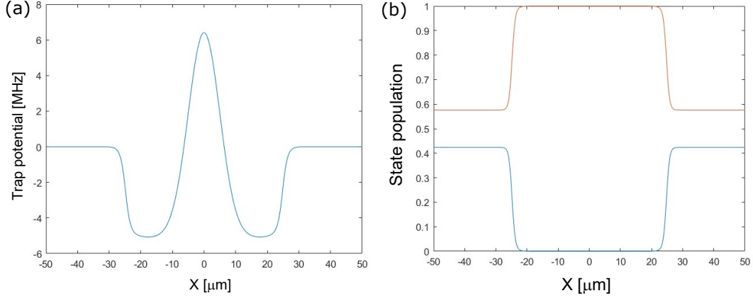
FIGURE 5.4 – (a) Calculation of the double dressed potential U_{tot}(x) in 1 dimension. (b) Population in the state 5p_{3/2} (blue) and in the state 5s_{1/2} (orange) versus the position of the atoms.
