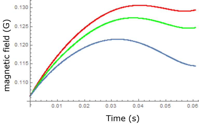
FIGURE 3.9 – Magnetic field seen by the K atoms in the +k_j configuration (green) and the -k_j atom interferometer (red). The field includes a temporal part common to the two trajectories and a spatial gradient which depends on the trajectory. The blue curve is the magnetic field measured with co-propagating Raman transitions, without any recoil modifying the trajectory.
