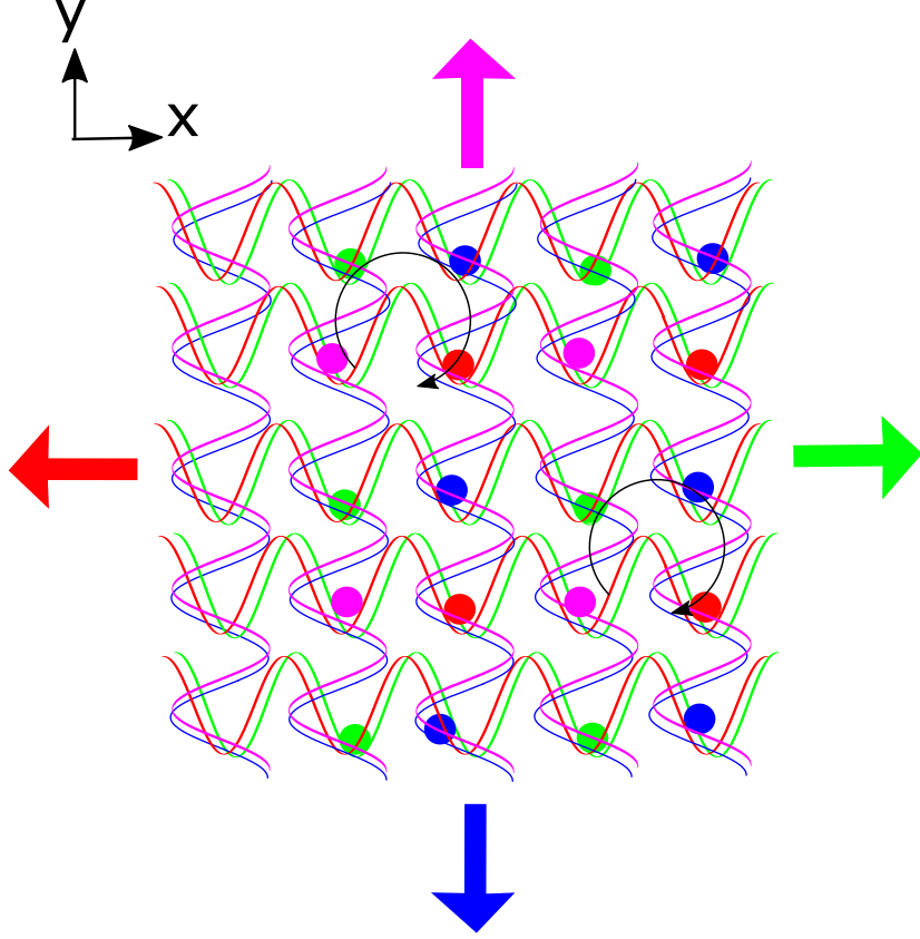
FIGURE 2.8 – The system is composed of 4 moving lattices going towards respectively +X (green), -X (red), +Y (magenta), -Y (blue). The atom in the state |0, +k_y\rangle (magenta full circle) is transported by the magenta lattice, then a 2D Raman pulse transfer it in the |-k_x, 0\rangle (red full circle) to be transported by the red lattice. The next step consists in a second 2D Raman pulse to transfer the atom in the |0, -k_y\rangle . Repeating the same process, each atom will follow a loop.
