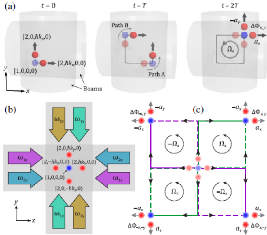
FIGURE 2.5 – (a) A sequence of atom-optical pulses constituting a 2D Mach-Zehnder interferometer. (b) A retroreflected beam geometry enabling 2D double-diffraction atom optics, which symmetrically transfer \hbar k_\mu of momentum along each axis \mu = x, y . (c) Four simultaneous 2D Mach-Zehnder AIs derived from the same atomic source. Linear combinations of the four phase shifts allow one to isolate the three inertial components a_x, a_y , and \Omega_z with increased sensitivity.
