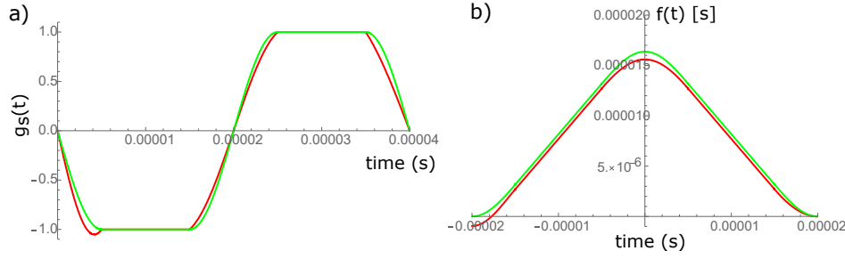
FIGURE 4.13 – Sensitivity function (a) and Response function (b) for an interrogation time T = 10\mu\text{s} , \tau = 5\mu\text{s} , \Omega_R^1\tau = \Omega_R^2\tau = \Omega_R^3\tau = \pi/2 (green) and \Omega_R^1\tau = 1.2\pi/2 , \Omega_R^2\tau = 0.8\pi/2 and \Omega_R^3\tau = 0.6\pi/2 (red). the small value of T is arbitrarily chosen for a good readability of the curve but have no connection with the reality of the experiments.
