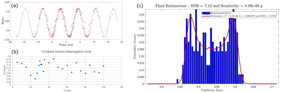
FIGURE 3.17 – (a) Fringes of a Mach-Zehnder atom interferometer achieved in microgravity on the zero-g simulator for an interrogation time 2T=20 ms. (b) Contrast of the atom fringes versus the interrogation time. (c) Histogram of the population ratio at the output of the interferometer for 2T=200 ms.
