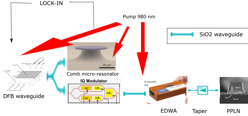
FIGURE 4.3 – Architecture of a miniaturized laser source based on telecom components and frequency doubling, integrated on a chip using SiO 2 PIC. The DFB laser is frequency lock using the reference coming from the comb generated by the ring micro-resonator. The IQ modulator developed by iXblue will generate all the required frequencies. The Erbium Doped Waveguide Amplifier will amplify the signal which is then frequency doubled in the PPLN waveguide. A common signal at 980 nm is used for the DFB, EDWA and the micro-resonator.
