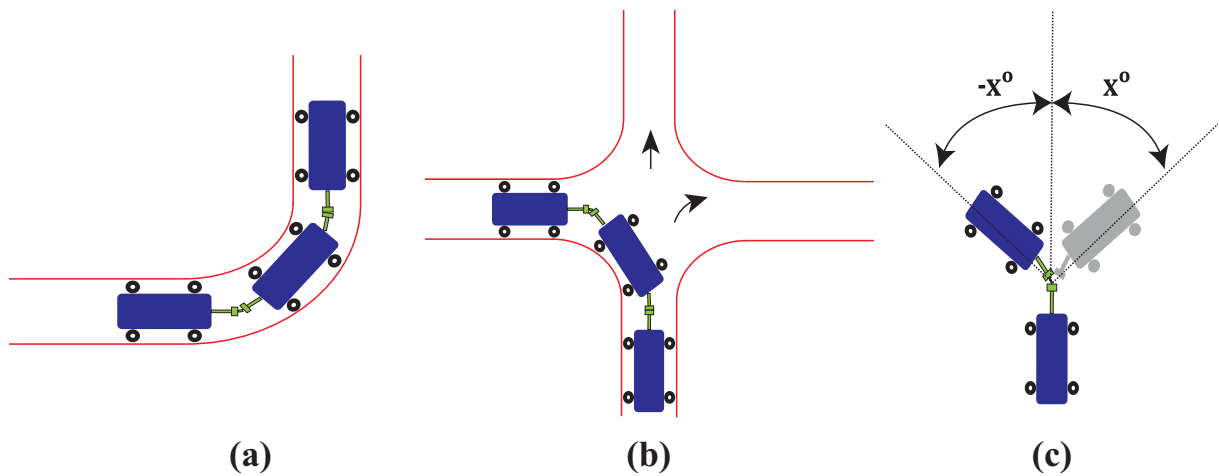
Figure 3.1 – Representation of (a) Passive compliance, (b) Active compliance and (c) Tilt limits for a piping inspection robot [VC19]
