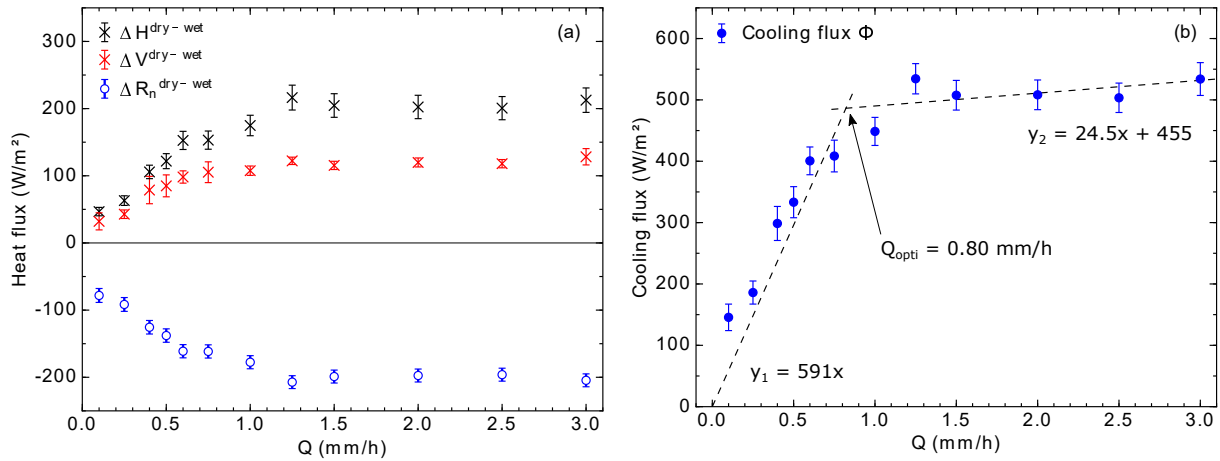
Figure 12.10: Dry-wet differences in net radiation \Delta R_n^{dry-wet} , in absorbed surface heat flux \Delta V_0^{dry-wet} and in atmospheric convective heat flux \Delta H^{dry-wet} (a), and total pavement cooling flux \Phi (b) to watering rate Q at the end of day phase. A double linear piecewise regression with zero-intercept is used on \Phi (b) (dashed lines) (Parison et al., 2020b).
