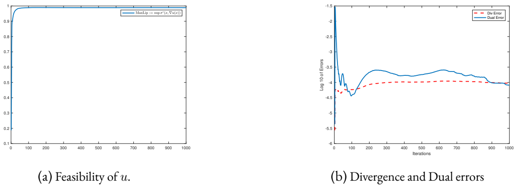
Figure 3.2: Error criterion for 1000 iterations with N_h = 120
