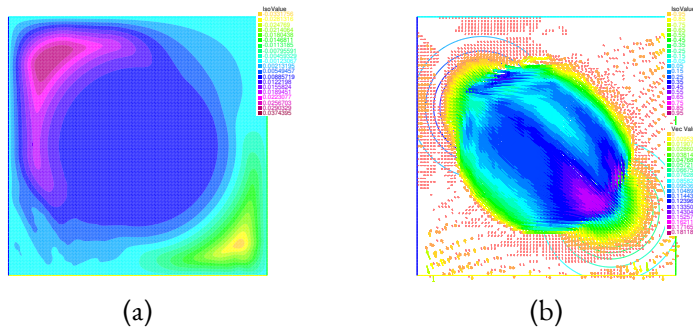
Figure 5.3: (A): the potential u , (B): the flow \phi privileging the zero set of k .
