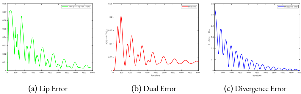
Figure 4.6: Error criterion for 5000 iterations and \tau = 0.01 and \eta = 8/\tau
