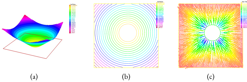
Figure 3.3: Left to right: 3D plot of the solution u , contour plot of u , the flux \phi
