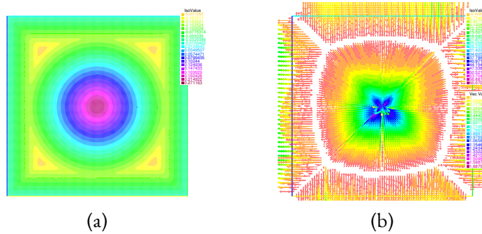
Figure 5.1: (A): the potential u , (B): the flow \phi .
