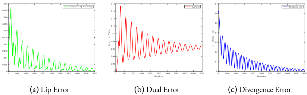
Figure 4.4: Error criterion for 5000 iterations and \tau = 0.01 and \eta = 8/\tau
