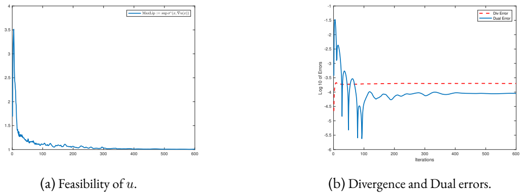
Figure 3.12: Error criterion for 600 iterations with N_h = 64 .
