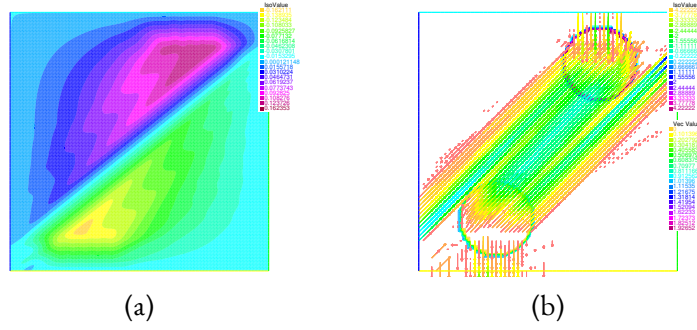
Figure 5.4: (A): the potential u , (B): the flow \phi .
