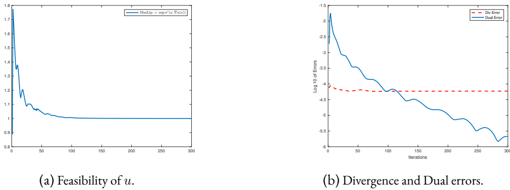
Figure 3.10: Error criterion for 300 iterations with N_h = 80 .
