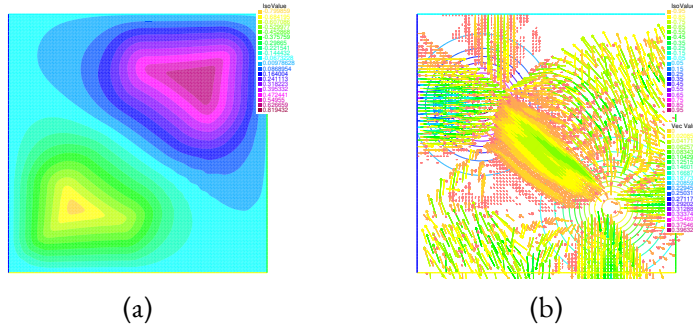
Figure 5.2: (A): the potential u , (B): the flow \phi .
