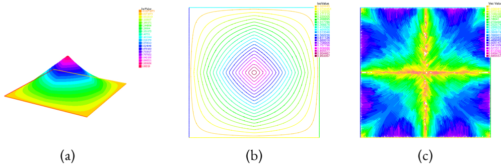
Figure 3.5: Left to right: 3D plot of the solution u , contour plot of u , the flux \phi
