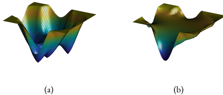
Figure 7.2: (A): the landscape height function g , (B): the constructed solution u .
