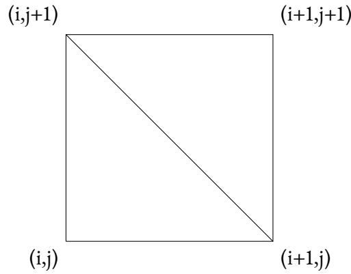
Figure 4.2: Sub-triangles
