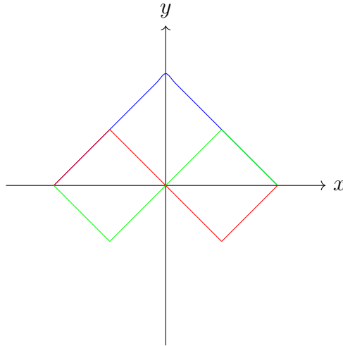
Figure 2.1: Several solutions of (2.3) on \Omega = (-1, 1) .
