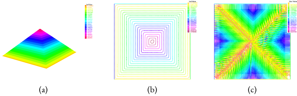
Figure 3.1: Left to right: 3D plot of the solution u , contour plot of u , the flux \phi
