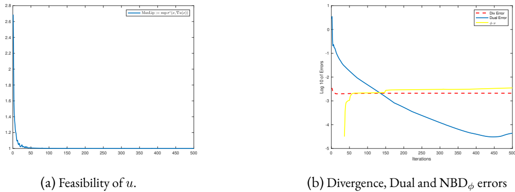
Figure 3.4: Error criterion for 500 iterations with N_h = 50
