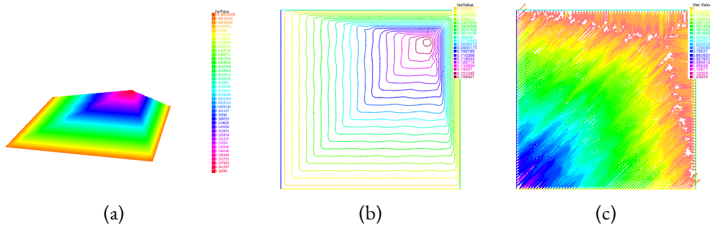
Figure 3.11: Left to right: 3D plot of the solution u , contour plot of u , the flux \phi
