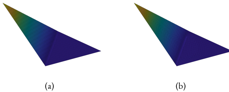
Figure 7.1: (A): the landscape height function g , (B): the constructed solution u .
