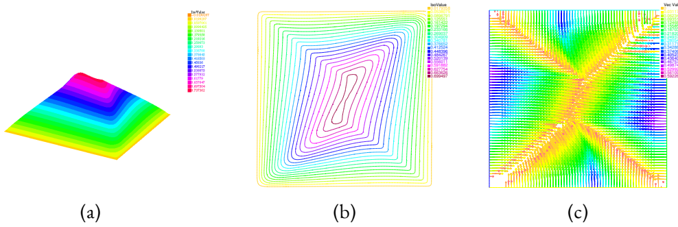
Figure 3.7: Left to right: 3D plot of the solution u , contour plot of u , the flux \phi
