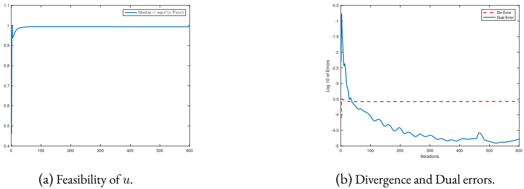
Figure 3.6: Error criterion for 600 iterations with N_h = 120
