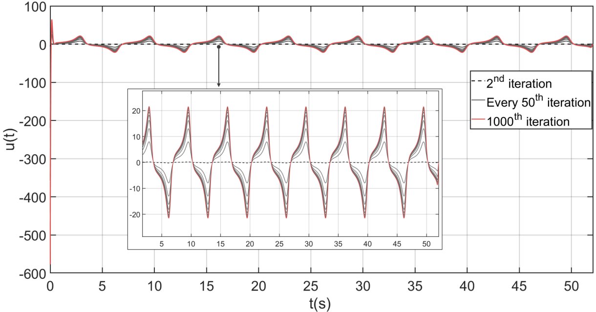
FIGURE 5.15: ILC inputs
