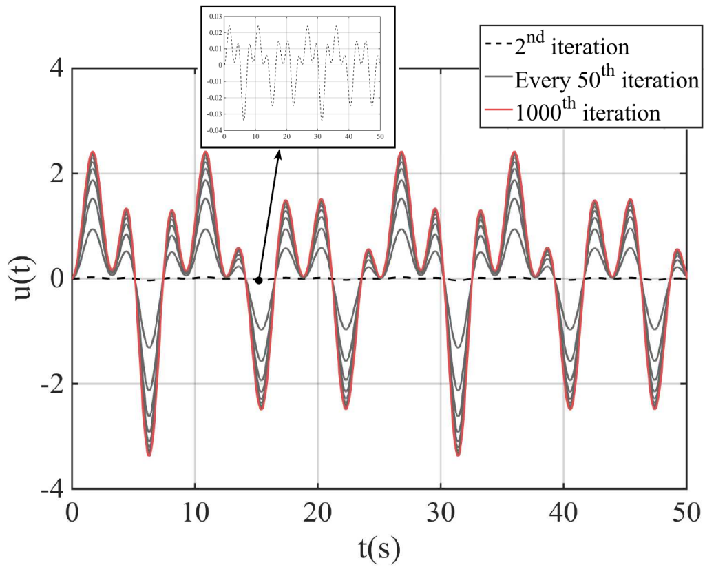
FIGURE 4.9: System input along iterations
