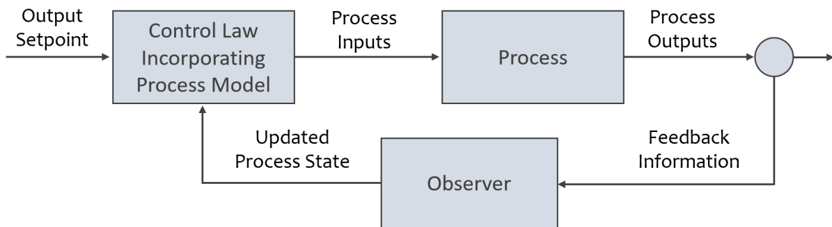
FIGURE 1.2: An example of a run-to-run controller [73]
