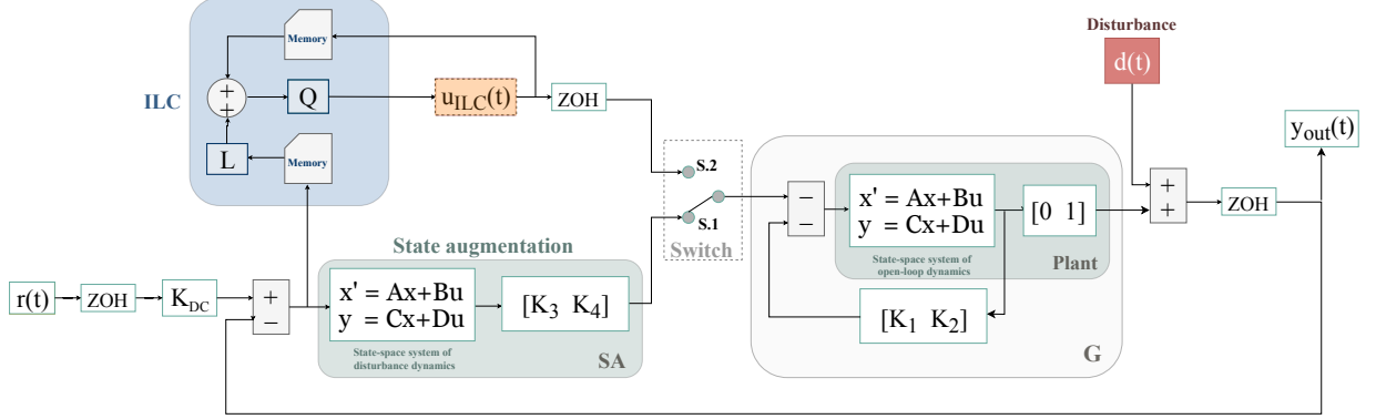
FIGURE 4.1: Simulation model
