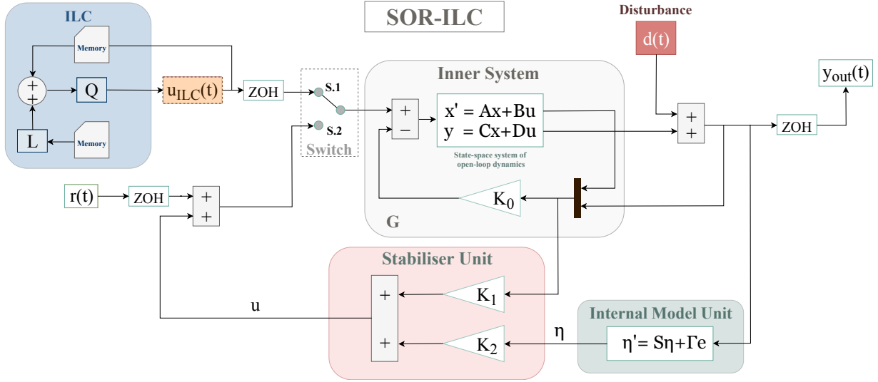
FIGURE 5.5: Simulation model
