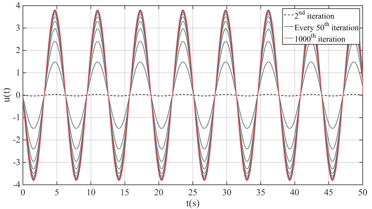
FIGURE 5.6: ILC inputs
