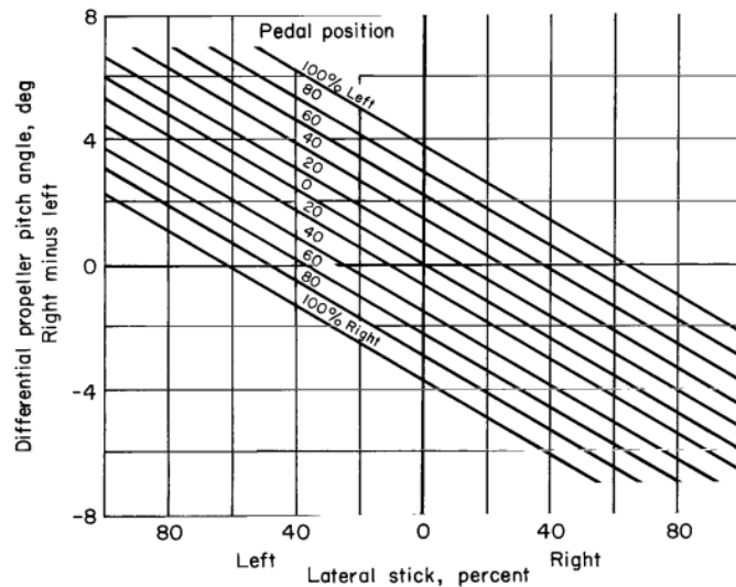
Figure 4 – Breguet Br-941 differential propeller pitch angle as function of pilot lateral (stick) and directional (pedal) inputs, reproduced from [Quigley 1964]
