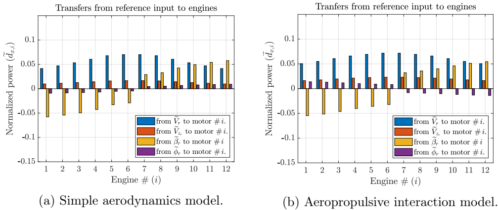
Figure 7.1 – Initial solutions allocation.
