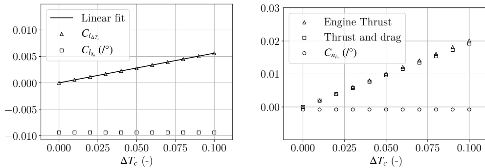
(a) Rolling moment induced by differential thrust compared with a 1° aileron deflection. (b) Yawing moment produced by differential thrust compared with a 1° rudder deflection.
