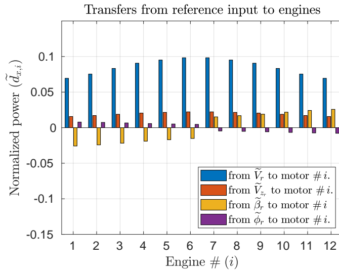
Figure 7.13 – Solution for the allocation after constrained co-design.
