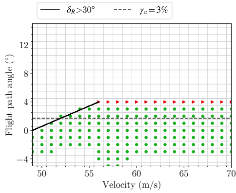
(e) DEP 4: Four right motors inoperative.
