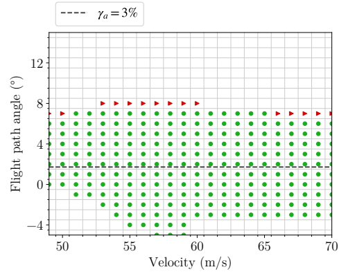
(b) DEP 1: One right motor inoperative.
