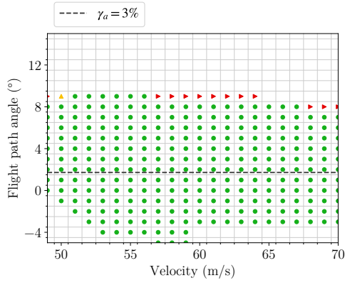
(a) DEP 0: All motors operative.
