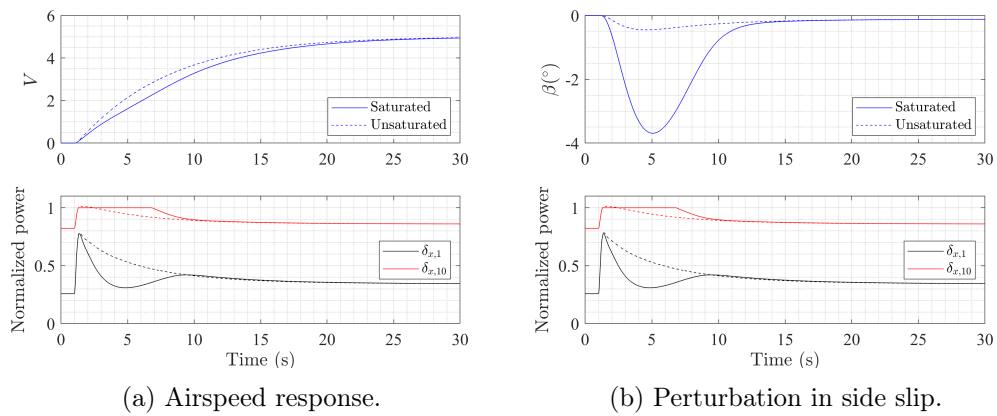
Figure 8.11 – Response to a V_r = 5 m/s step input in asymmetric conditions. Dashed line: with unsaturated actuators, continuous line: with saturated actuator.
