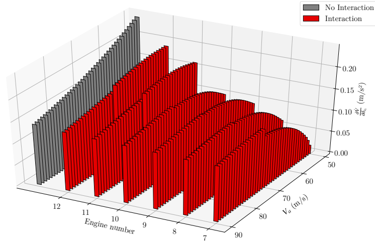
(a) \frac{\partial \dot{V}}{\partial \delta_{x,i}} at 7.5^\circ flap deflection.
