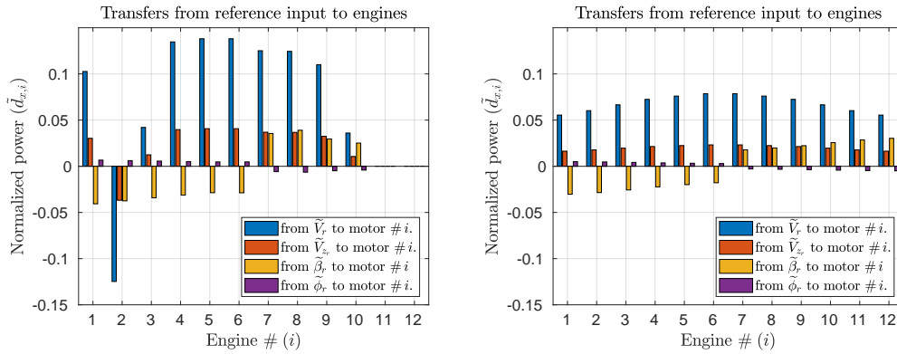
(a) Solution for the allocation in asymmetric thrust conditions. (b) Solution for the allocation in nominal thrust conditions.
