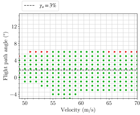
(c) DEP 2: Two right motors inoperative.
