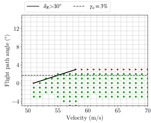
(f) DEP 5: Five right motors inoperative.
