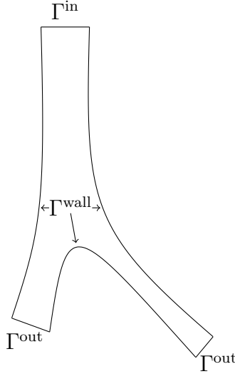
Figure 6.2: Domain \Omega
