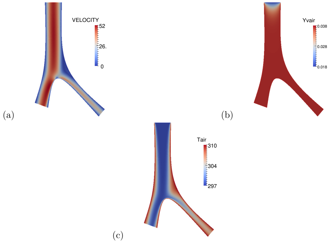
Figure 6.3: Distribution of (a) the velocity |u| , (b) the water vapor mass fraction in the air Y_{v,\text{air}} and (c) the temperature T_{\text{air}} at the final time \tau = 1 s.
