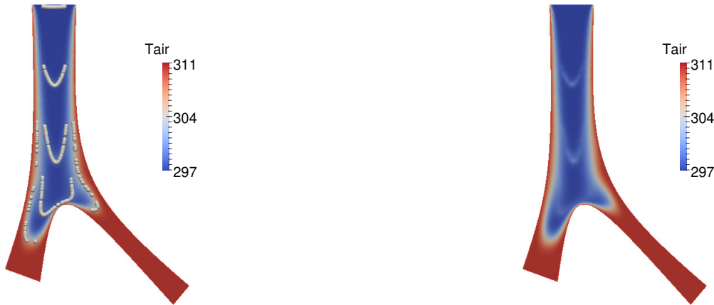
Figure 6.6: Local effects of the aerosol on the air temperature at time 0.25 + \Delta t (in seconds), with the plot of the particles (left) and without (right).
