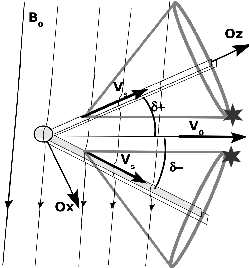
Figure 4.5: Alfvén wings attached to the pulsar companion, immersed in the pulsar magnetic field. Each wing forms an angle \delta_{\pm} with respect to the radial direction (i.e radial outflow velocity). The velocity of the source regions \vec{v}_s is assumed to be along the Alfvén wings. From which, the cones represented by the thick grey lines, describe the radio emission directions. The two stars show the highest emission intensity directions of each wing. Taken from [227].
