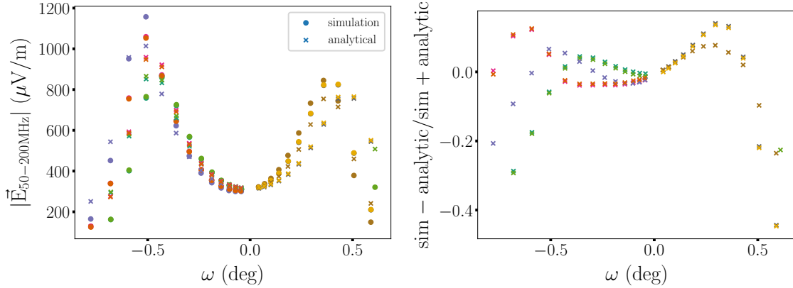
Figure 3.36: Left: Illustration of the full signal amplitude distribution for antennas above 5\sigma_{\text{Amp}} = 110\mu\text{V/m} as in the simulation trigger conditions. The model correctly describes the general trend but fails to accurately reproduce the exact value of the simulation data. Signals computed for a EAS with azimuth 180^\circ , zenith 92.92^\circ , primary proton of energy 3.94\text{EeV} . Right: Display of the residuals computed as (\text{simulation} - \text{model}) / (\text{simulation} - \text{model}) .
