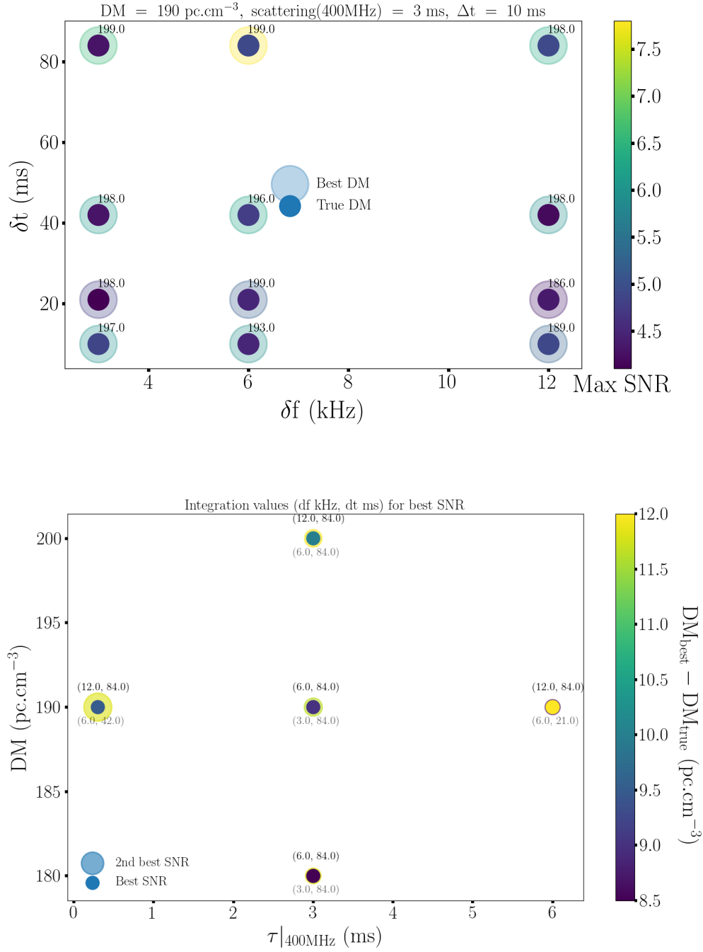
Figure 5.9: Study of the effects of the observation parameters on the detected SNR of FRB signals. Top: Evolution of the SNR, for various frequency and time resolution, corresponding to the true DM or the best DM. Bottom: Evolution of the difference between the true DM and the best DM as a function of the DM and scattering time \tau , with the corresponding best SNR and second best SNR for the corresponding observation parameters. High resolutions (in time and frequency) are not required to detect FRB signals with high SNR, therefore a reasonable resolution of (21 ms, 3 kHz) can be chosen as a compromise between space storage convenience and flexibility in the analysis (post integration of signals in order to find the true DM).
