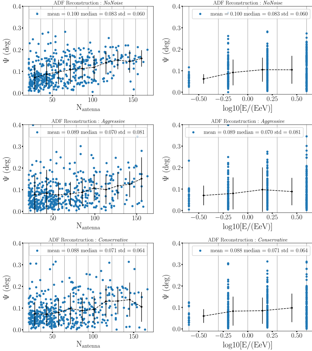
Figure 3.51: Left column: Angular distance \psi as a function of the number of triggered antennas N_{\text{ant}} . Right: Energy dependancy of the angular distance \psi . Top: For the NoNoise scenario. Middle: For the Aggressive scenario. Bottom: For the Conservative scenario. For the GP300-like layout.
