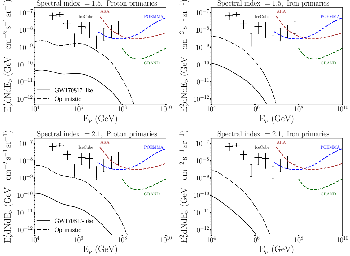
Figure 1.12: Diffuse neutrinos spectra for injection spectral index \alpha = 1.5 (top) and \alpha = 2.1 (bottom) of proton primaries (left) and iron primaries (right), with baryon loading \eta_p = 0.1 . The GW170817-like scenario follows a flat source evolution with rate \dot{n}_0 = 600 \text{ Gpc}^{-3} \text{ yr}^{-1} , while the optimistic scenario follows a SFR source evolution with rate \dot{n}_0 = 3000 \text{ Gpc}^{-3} \text{ yr}^{-1} .
