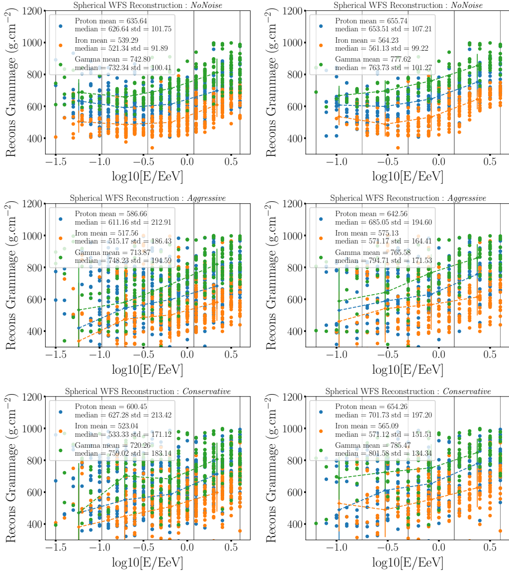
Figure 3.55: Reconstructed grammage as function of the primary energy. Left column: without quality cuts. Right column: with quality cuts ( N_{\text{ant}} > 15 units and \theta < 115^\circ ).. or the Star-Shape simulation set. Top: For the NoNoise scenario. Middle: For the Aggressive scenario. Bottom: For the Conservative scenario.
