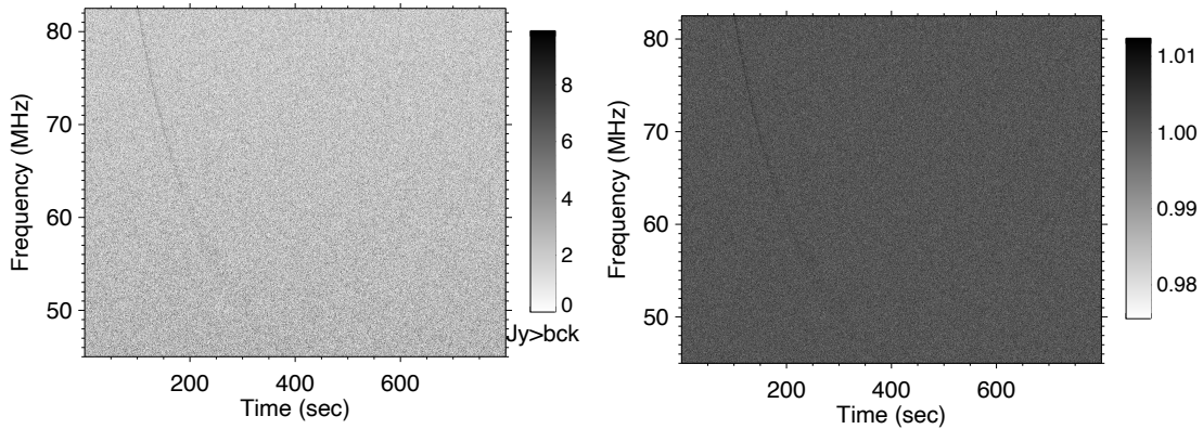
Figure 5.4: FRB simulated signal observed by 96 MA in the time-frequency plane for a frequency and time resolution of df = 3 kHz and dt = 21 ms, taking into account the sky background noise. Left : without any correction. Right : with spectral flattening to correct for the spectral slope induced by the galactic noise (see Section 5.2.3.2).
