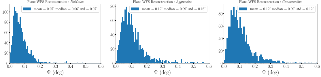
Figure 3.37: Histograms of the angular distances \psi plane wave reconstruction for the Star-Shape simulation set. Left: for the NoNoise scenario. Middle: for the Aggressive scenario. Right: for the Conservative scenario.
