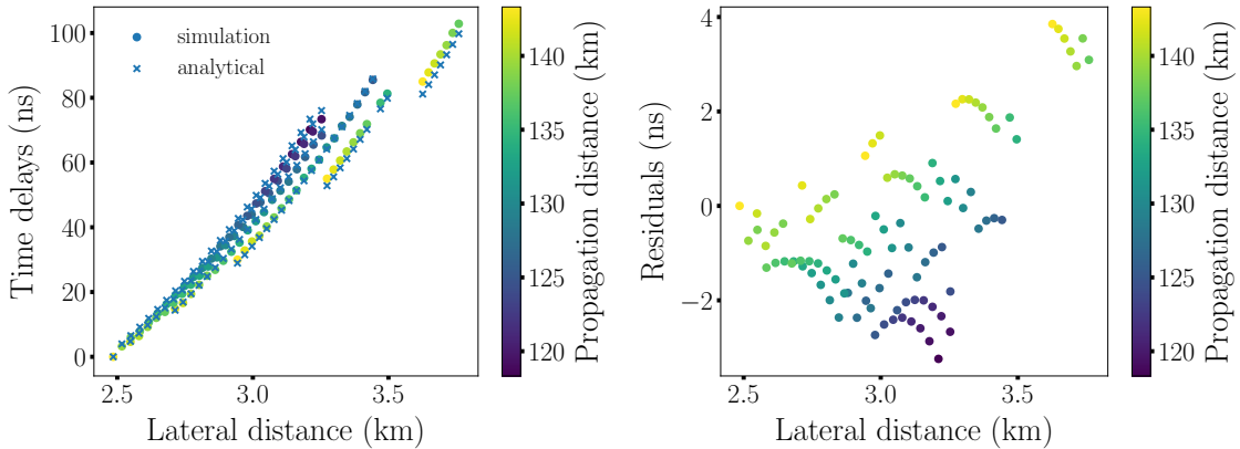
Figure 3.21: Left: Trigger times with respect to the propagation plane, as a function of the distance to shower axis. The time delay computed for the analytical spherical model are shown as blue crosses. Right: Residuals of the difference between the simulation data and the spherical model.
