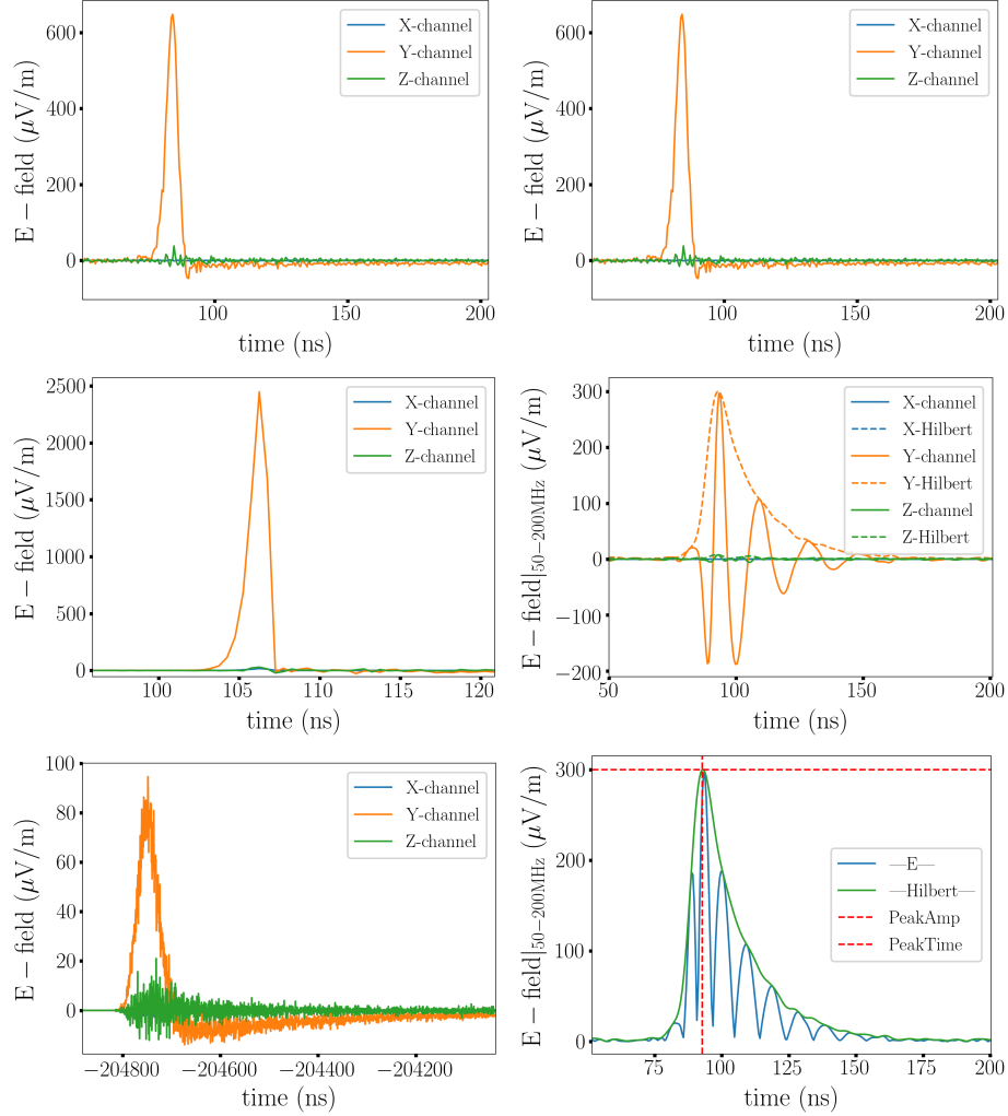
Figure 3.2: Left column: Exemples of simulated electric field traces for various locations inside the footprint (note here the different time and amplitude scales). Top: inside the Cerenkov cone (2.9 km from the shower core). Middle: at the Cerenkov cone (3.4 km from the shower core). Bottom: Outside the Cerenkov cone (61.7 km from the shower core). As it can be clearly seen, closer to the Cerenkov cone the signal amplitude rises while the time width of the signal tightens. The signals were simulated for a proton induced EAS of energy 3.94 EeV, azimuth 180^\circ and zenith 92.92^\circ . Right column: Exemple of ZHAireS simulated signals as seen by an antenna. Top: Raw electric-field signal at the antenna location. Middle: Filtered electric-field and Hilbert envelope of each channel (see Section 3.2.3.1). Bottom: Modulus of the electric field and of the Hilbert envelope. The maximum of the Hilbert envelope is used as a definition of the trigger time and peak-amplitude in our study. For a proton induced EAS of energy 3.94 EeV, azimuth 180^\circ and zenith 92.92^\circ .
