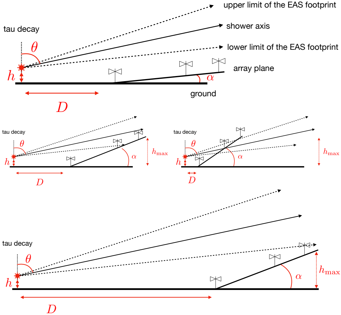
Figure 2.19: Various illustrative sketches of the impact of the toy-model topography on the detection of an up-going EAS. Four scenarii are considered here: Top: A low inclination results in a total loss of the signal as the emission flies above the array. Middle left: A sufficient inclination leads to a detection of the signal as several antennas intercept the emission. Middle right: A close-by detector from the tau decay point intercepts the emission, however the footprint on the array is too small to contain enough antennas to issue a trigger. Bottom: A detector far away from the tau decay point misses the signal since no interception of the emission can be achieved due to the altitude limitation of the array. As illustrated here, an optimal parameter set for the topography of the detector lies in arrays inclined of a few degrees and distant of a few tens of kilometers from the tau decay point.
