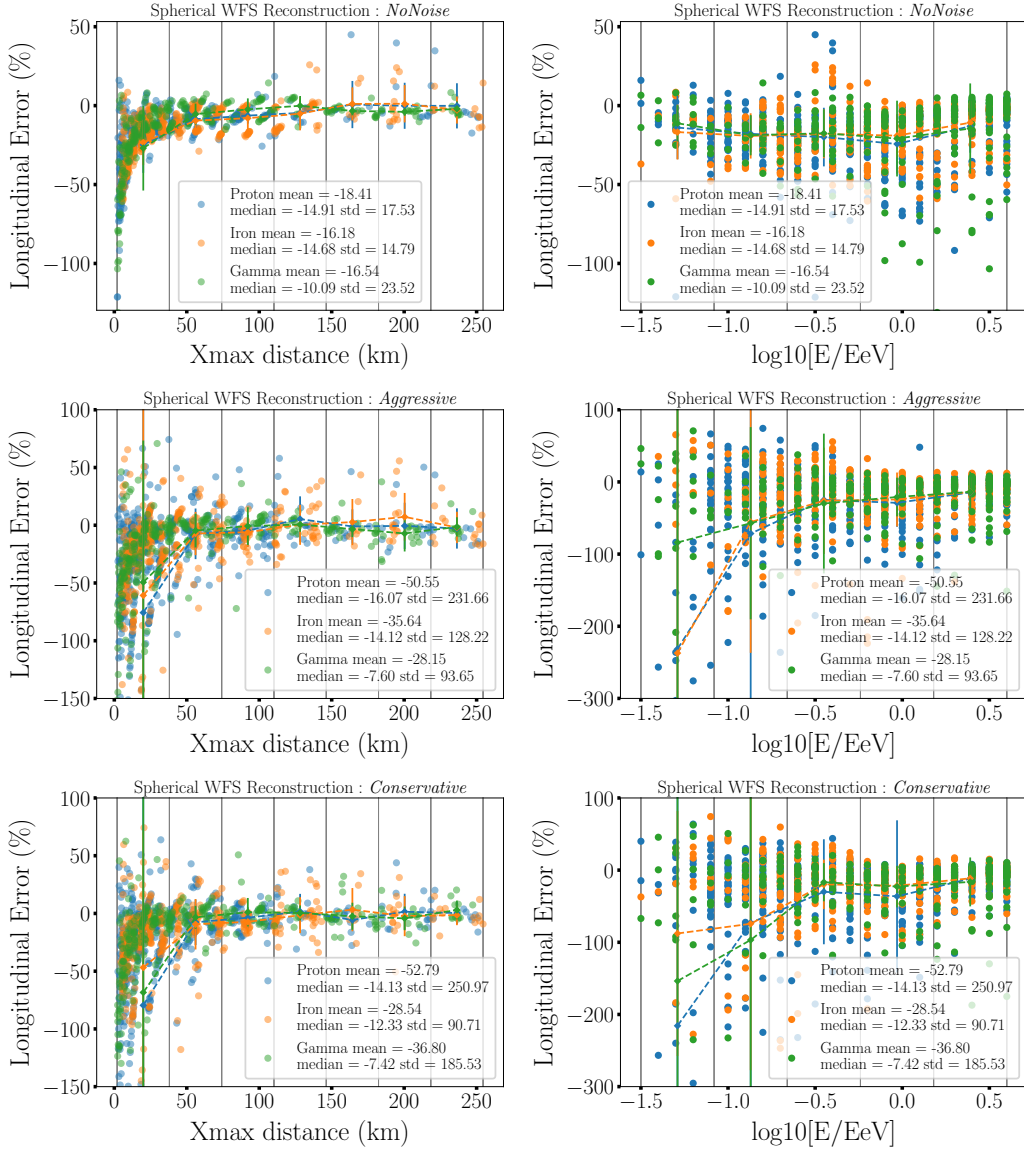
Figure 3.41: Lef column: Relative longitudinal error on the reconstruction of the source position as function of the X_{\max} distance to the shower core. Right column: Relative longitudinal error on the reconstruction of the source primary energy. For the Star-Shape simulation set and with a reference set at X_{\max} . Top: For the NoNoise scenario. Middle: For the Aggressive scenario. Bottom: For the Conservative scenario.
