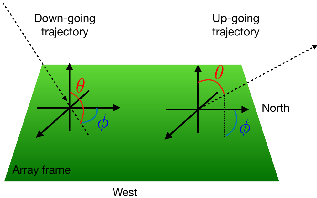
Figure 2.1: Sketch of the GRAND angular conventions. The reference frame is colocated with the array frame, resulting in up-going trajectories with zenith angles defined as 0^\circ \leq \theta \leq 90^\circ , and thus down-going trajectories have zenith angles such that 90^\circ \leq \theta \leq 180^\circ . Finally, the origin of the azimuth is oriented toward the North and counting clockwise toward the West.
