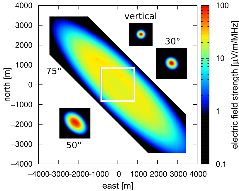
Figure 3.9: Sizes of simulated footprints on ground for various zenith inclinations (cosmic-ray conventions). The footprint grows strongly with the zenith inclination up to kilometer-size areas. For showers close to 90^\circ , footprints even extend to several tens of kilometers. Taken from [176].
