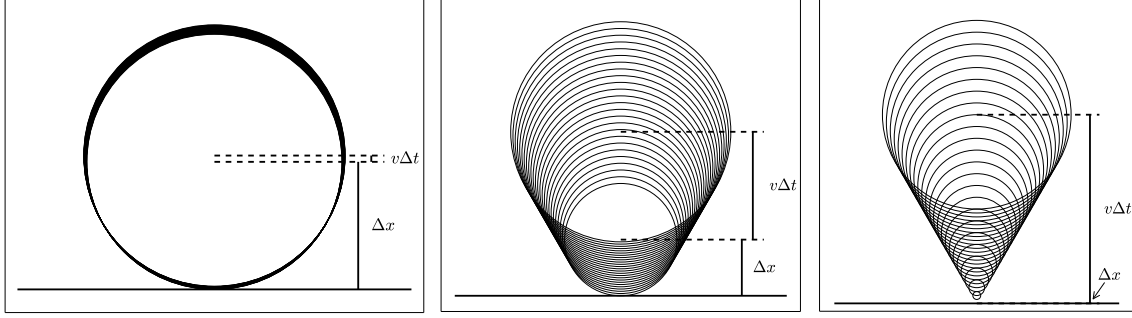
Figure 3.6: LOFAR wavefront models. Each of them corresponds to a specific configuration of emission region of size \sim v\delta t compared to propagation distance \Delta x . Left: Spherical wavefront model corresponding to v\delta t \ll \Delta x . Middle: Intermediate case where the emission region extension v\Delta t \sim \Delta x creates a deviation from the spherical wavefront i.e. hyperbolical curvature. Right: Extreme case where the emission region v\Delta t \gg \Delta x dominates the propagation distance leading to a conical wavefront emission detected. Taken from [24].
