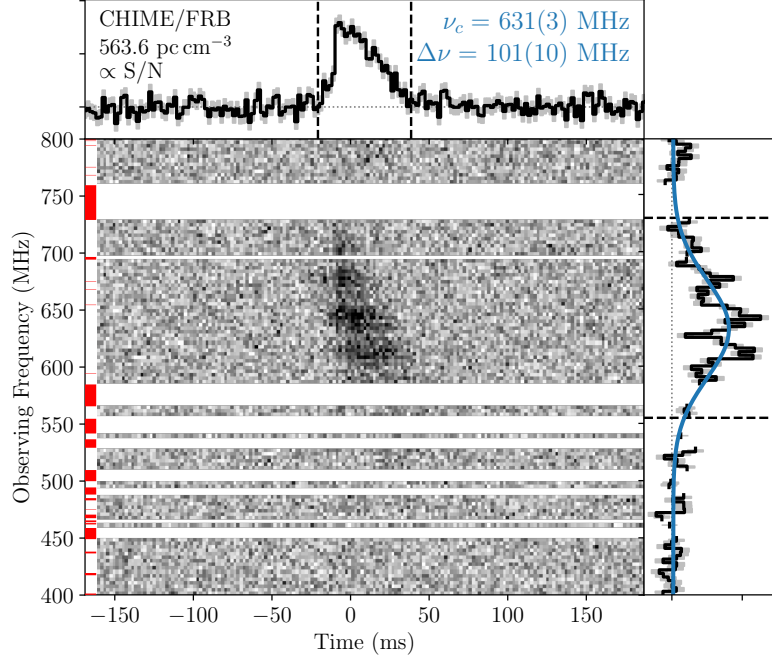
Figure 4.2: Dynamic spectrum ( Center ) and waterfall plots along the time ( Up ) and frequency dimension ( Right ) for the Arecibo repeater FRB121102, observed for the first time around 600 MHz with the CHIME telescope. A clear frequency broadening effect can be observed towards the low frequencies, which is not present at the Arecibo observatory frequency. Taken from [220].
