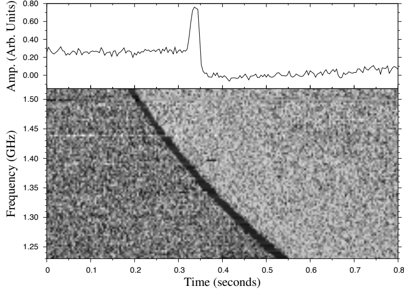
Figure 4.1: The Lorimer burst, the first detected FRB in 2007. Top : Waterfall plot (projection along the temporal dimension of the dynamical spectrum of the de-dispersed signal) of the pulse, integrated along the frequencies. Down : Dynamical spectrum of the pulse. The pulse can be characterised as a milliseconds pulse over a broad band frequency range. Furthermore the large time delay between the high frequencies and the low ones clearly shows a signal with a high DM. Taken from [219].
