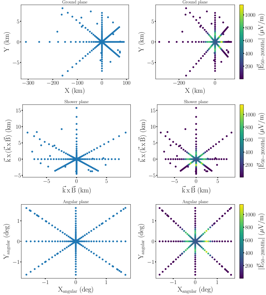
Figure 3.7: Left column: Star-Shape antenna layout. Antennas are placed at regular angles from the shower direction (here flying towards the South, azimuth= 180°) along the star-shape pattern. The x-axis and y-axis stand respectively for the South-North and East-West directions. This layout results in an stretched ellipsoidal star-shape along the shower direction on ground ( Top ) and therefore also in the shower plane ( Middle ). However in the angular plane ( Bottom ) the star-shape is by definition a symmetric circle, which makes this frame convenient for the study of inclined EAS (see Figure 3.8 for a sketch). Right column: Illustration of the signal amplitude distribution on ground of a Star-shape EAS simulation for azimuth 180° flying towards decreasing values of the x-axis, zenith= 92.92° and primary proton energy 3.98 EeV. Top: In the array plane. One can see the clear ellipse pattern. Middle: In the shower plane. The amplitude pattern is still an ellipse event though the projection attenuates it. Bottom: in the angular plane, where all projection effects are naturally corrected. Some antennas have been randomly placed outside the star shape for verification purposes when the simulation set was produced. We keep these antennas for the following study.
