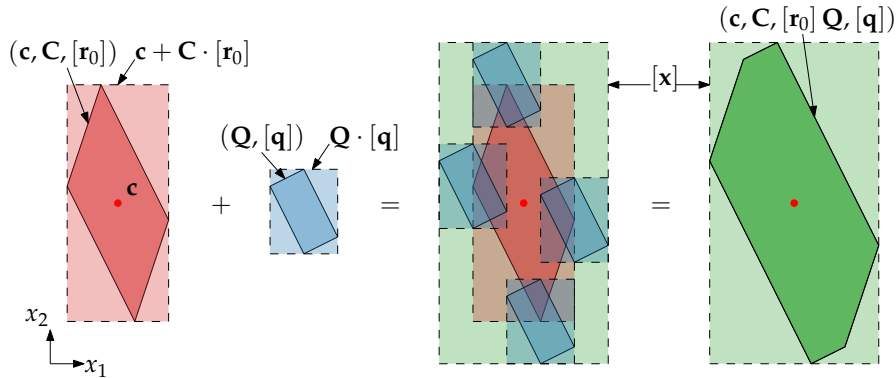
Figure 2.16: Representation of a cuboid-based doubleton
