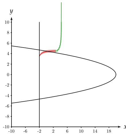
(c) Trajectory initialised at \mathbf{x}_0 = E : after leaving the first state q_0 , the system will never cross the parabola.
