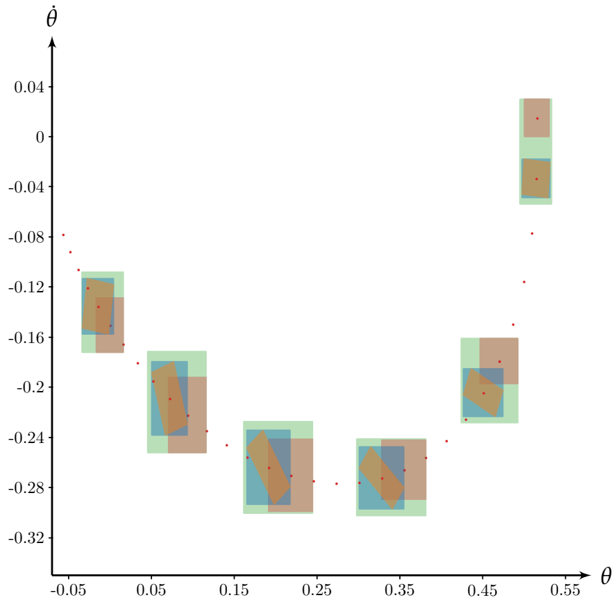
Figure 2.23: Integration of a simple pendulum by Algorithm 2
