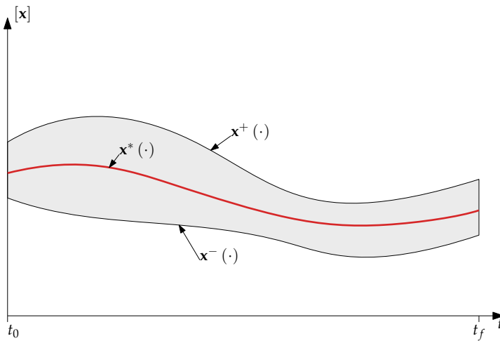
Figure 4.1: Illustration of a one-dimensional tube
