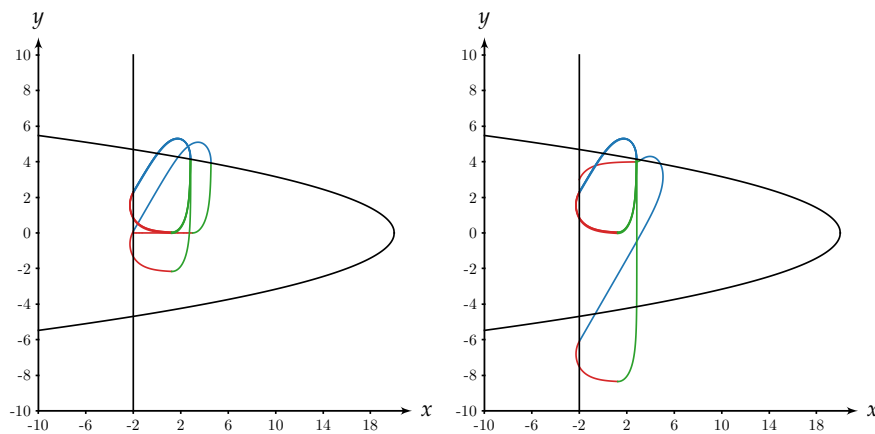
(a) Trajectory initialised at x_0 = B (b) Trajectory initialised at x_0 = D
