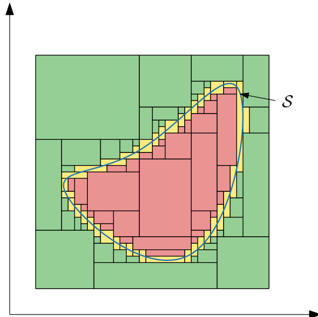
Figure 2.27: Inner and outer paving of a set \mathcal{S} : red boxes are inside \mathcal{S} , green ones outside, and nothing can be said about yellow boxes
