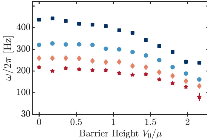
Figure 7.9. – Frequencies of the Josephson oscillations at different barrier heights for box sizes of 15\mu\text{m} (blue squares), l_x = 20\mu\text{m} (blue circles), 25\mu\text{m} (orange diamonds) and 30\mu\text{m} (red stars). At vanishing barrier height, the frequencies are determined by the speed of sound and are proportional to 1/l_x . The frequencies decrease for increasing barrier height. Oscillations are visible up to barrier heights of V_0 > 2\mu .
