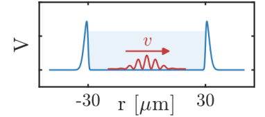
Figure 7.13. – Sketch of the perturbation scheme of the 2D gas. A lattice potential (red) is imprinted from the top into the homogeneous gas. By detuning the two lattice beams, the lattice moves at an adjustable velocity v . The lattice constant can be tuned by adjusting the crossing angle of the two incident beams. Figure adapted from [226]
