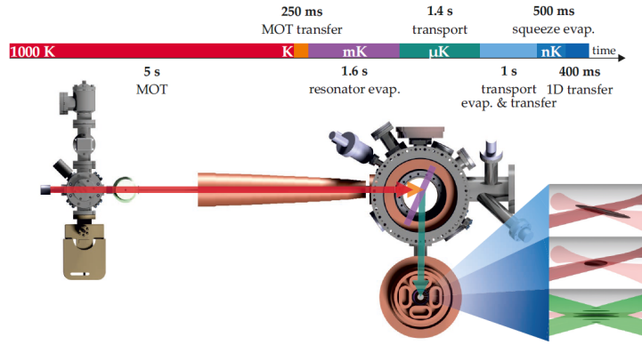
Figure 5.11. – Summary of the experimental procedure for the preparation of a 2D Fermi gas (adapted from [134]). (Red arrow) The atomic beam exits the oven and is decelerated in the Zeeman slower. The atoms are trapped in a MOT which is loaded in about 5s. After saturation of the atom number, the MOT is shifted to the resonator loading position and the atoms are transferred into a deep standing wave potential inside an in-vacuo resonator (purple). A first evaporative cooling step takes place and the atoms are subsequently loaded into a running wave optical dipole trap. Over 1.4 s, the focus of this trap is moved forward (green arrow) and the atoms are transported into the science cell. Here, the gas is loaded into the highly elliptic squeeze trap (inset pic. 1,2), which flattens the cloud to a vertical size of \sim 1 \mu\text{m} . Finally the gas is loaded into the repulsive optical lattice (inset pic. 3), which confines the gas to the quasi-2D regime.
