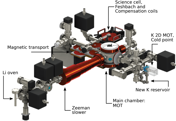
Figure 3.1. – CAD drawing of the Fermix vacuum system. The apparatus consists of two source regions, a lithium oven and a potassium 2D MOT which connect to an octagonal central cell (via a Zeeman slower in the case of lithium). Here the atoms are captured and cooled optically. In order to transfer the atoms into a region of high vacuum quality and large optical access, a magnetic transport links the main chamber to the science cell. For clarity, the top coils of the transport and the science cell region are not shown. Figure adapted from [104].
