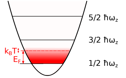
Figure 2.4. – Energy diagram of a two-dimensional gas. A gas is in a quasi-two-dimensional configuration if the level spacing of the strongly confining potential is larger than all other relevant energy scales, such as the thermal energy k_B T or the Fermi energy E_F . In this case, the atoms occupy the motional ground state in the direction of strong confinement.
