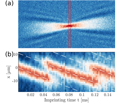
Figure 7.8. – Imaging the phase difference of the 2D gas in the box: The momentum distribution is accessed by letting the atoms evolve freely for a quarter period in an underlying weak harmonic potential, which in equilibrium yields a peak at k = 0 . (a) During this evolution, the atoms quickly expand along the vertical direction, forming a cigar-shaped cloud whose upper and lower parts are out of focus of our microscope objectives. By tilting the imaging beam slightly with respect to the vertical, the unfocused upper and lower parts of the column are shifted to the left or right on the image, whereas the focused central part is now visible in the center of the image. We use the central slice (red box) to fit the position of the central peak. (b) Calibrating the phase measurement: By imprinting the repulsive potential for different times, we imprint different phase differences onto the two sides of the box. The image shows the central slices of the momentum distribution measured as described above for the different phase imprints \Delta V_{\text{pulse}} t . For increasing imprinting time, the position of the pair condensation peak shifts in space linearly, showing a periodic pattern with a period of \varphi_0 = 2\pi \approx 7\text{ ms} . This displacement pattern is used to calibrate the initial phase imprint for the experimental sequence. The displacement of the peak is also used to measure the phase difference during the Josephson oscillations.
