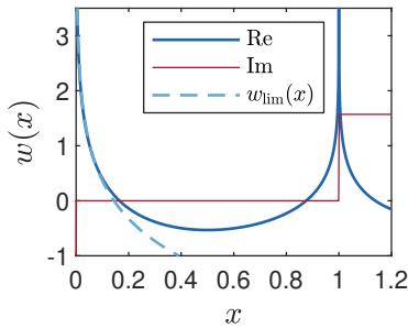
Figure 2.6. – Real and imaginary parts of the function w(x) defined by 2.34. The range of validity x < 0.1 of the approximation w_{\text{lim}}(x) (light blue) defines the quasi-2D regime.
