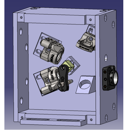
Figure 5.15. – Open view of the beam splitter optics. The beam enters the box through the front wall (not shown) and is reflected up and then downward using two fixed mirrors into the polarizing beam splitter (yellow). The two resulting beams are reflected out of the right hand side of the box via two mirrors, which can be adjusted via holes in the back plate of the box. The lower beam passes a wave plate which rotates its polarization to match the polarization of the other beam. After the wave plate the remaining optical path length is the same for both beams.
