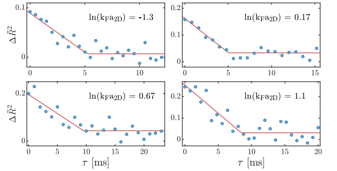
FIG. S3. Superfluid phase transition at different interaction strengths. Difference \Delta \bar{R}^2 of the adjusted coefficients of determination between fits to r(v, T) with zero and non-zero v_c as a function of heating time \tau for different interaction strengths. Linear fits of \Delta \bar{R}^2 with a threshold at a critical heating time (red lines) clearly show the appearance of a non-zero critical velocity below a critical temperature for systems across the crossover (A,B,C) and into the BCS regime (D). However, due to the challenges involved in measuring the temperature of strongly interacting homogenous Fermi gases discussed in the text we are currently not able to quantitatively determine the relation between the heating time and the temperature for these systems and hence cannot give a value for T_c .
