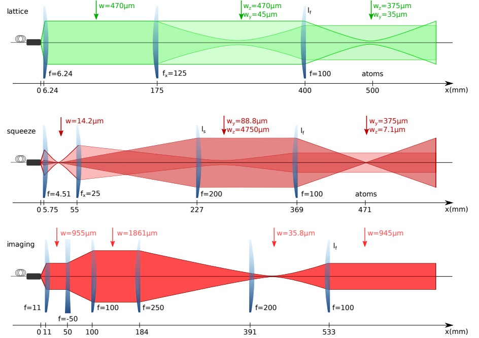
Figure 5.14. – Parameters of the optical setups on the new breadboard. The lattice beam is split into the two paths after the first collimating lens, which is not shown here. The second lens in the lattice and squeeze setups are cylindrical lenses, creating the elliptic beam profiles. The imaging and squeeze are overlapped on a back-polished mirror and share the two final lenses. The two beams are then overlapped with the lattice beams on a dichroic mirror. All beams share the same final high precision doublet lens f_i (Melles Griot LAI-100.0-30.0). The beam waists and distances of the three diagrams are not drawn to the same scale. For the squeeze schematics, the scale vertical beam axis is reduced by a factor 5 with respect to the horizontal axis to draw them in the same diagram.
