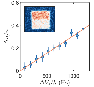
Figure 6.5. – Static measurement of the compressibility. A repulsive potential V is imprinted onto one half of the box resulting in a density imbalance \Delta n/n (blue points). We extract the compressibility from the initial slope of the data points according to 1/n^2\kappa = \lim_{\Delta n \rightarrow 0} \Delta V_s/\Delta n in a local density approximation. Each data point and the inset are averages of 20 realizations.
