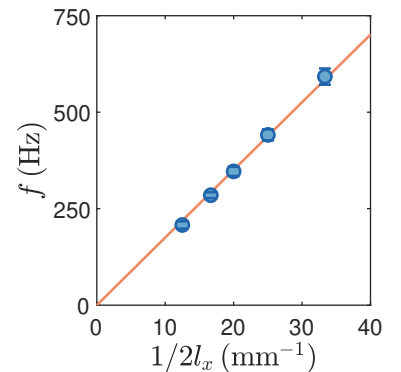
Figure 6.2. – Frequency of the density oscillations as a function of the inverse box length. The slope of the linear fit (solid line) corresponds to the speed of sound. Each data point is the average of 23 realizations.
