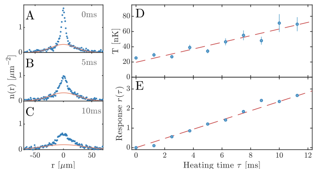
FIG. S2. Calibration of the heating procedure. (A-C) Measurements of the momentum distribution of the gas after applying the moving lattice to the system for different heating times \tau . The red solid lines show the Boltzmann fits to the wings of the distribution from which the temperature is extracted. (D) Temperature T of the gas as a function of heating time. We observe that the temperature of the gas increases roughly linearly with the heating time (red dashed line). (E) Response r(\tau) as a function of heating time. The response shows a very similar behavior to the temperature, but can be measured with a much higher signal-to-noise ratio. All data points are obtained from an average of 55 individual measurements. The error bars in (D) denote the 1\sigma confidence interval of the fit.
