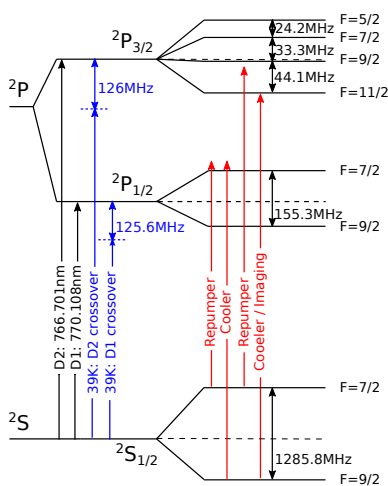
Figure 3.2. – Level scheme of fermionic potassium and of the optical transitions used at Fermix. The energy splittings are not to scale. The D1- and D2-lines between the 4^2S_{1/2} ground state and the 4^2P_{1/2} and 4^2P_{3/2} excited states are both used in the Fermix element. The lasers are locked onto the respective crossover lines of ^{39}\text{K} , which are offset by only about 125 MHz with respect to the lines of ^{40}\text{K} . For the MOT and the D1-molasses, bichromatic beams consisting of a cooling and repumping frequency are used, in order to prevent an unwanted accumulation of atoms in the |F = 7/2\rangle ground state.
