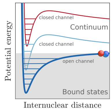
Figure 2.5. – Schematic representation of a Feshbach resonance. Two atoms are colliding in the continuum of an open channel (dark blue). The interaction between the spins admixes contributions of different spin wavefunctions. These are subject to different interaction potentials (light blue, red). Due to the different magnetic momenta of these different spin configurations, the energy difference between the potentials can be tuned. When the energy of bound state becomes resonant with the energy of the colliding atoms, the scattering amplitude becomes strongly enhanced. Since the atoms could not escape to infinite distance in the light blue and red potentials, these channels are said to be closed.
