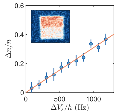
Figure 6.5. – Static measurement of the compressibility. A repulsive potential V is imprinted onto one half of the box resulting in a density imbalance \Delta n/n (blue points). We extract the compressibility from the initial slope of the data points according to 1/n^2\kappa = \lim_{\Delta n \rightarrow 0} \Delta V_s/\Delta n in a local density approximation. Each data point and the inset are averages of 20 realizations.
