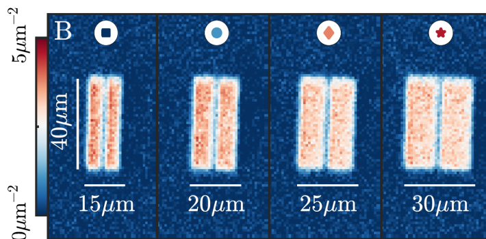
Figure 7.7. – Examples of Josephson junctions in 2D gases with different geometries. As before, we denote with l_x the direction of the oscillations, and with l_y the direction perpendicular to l_x , determining the length of the barrier.
