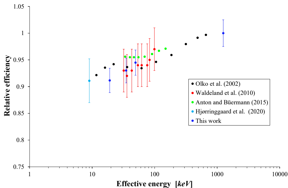
FIGURE 5.21: Comparison of \eta^{Q,Q_0} values obtained with Monte Carlo (MC) simulations with published data.
