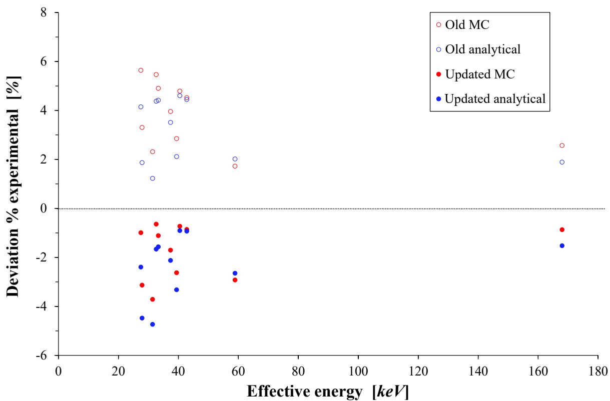
FIGURE 5.23: Comparison of preliminary and updated f_{MC}^{Q,Q_0} and f_W^{Q,Q_0} factors with experimental f_{exp}^{Q,Q_0} values.
