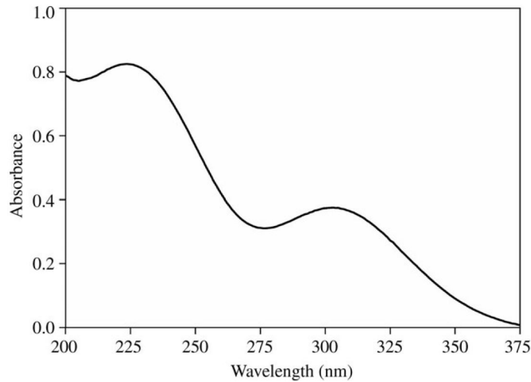
FIGURE 3.10: Absorption spectrum for a Fricke solution irradiated at 100Gy. (Optical path length = 1cm)[67]
