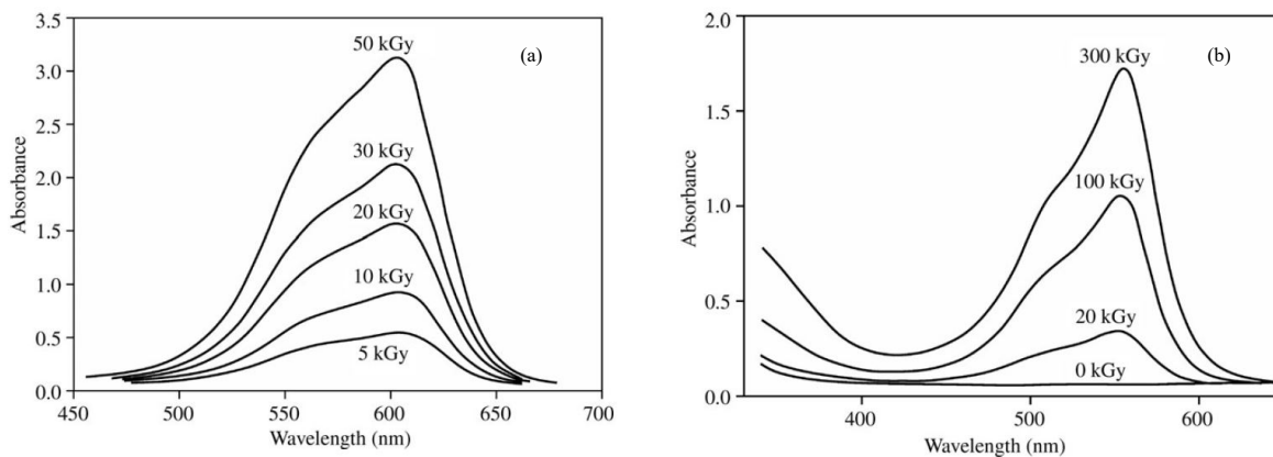
FIGURE 3.8: Typical measured absorbance spectra of both (a) FWT-60 and (b) B3-Risø dosimeters, as a function of wavelength.
