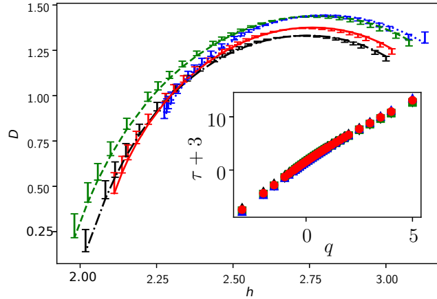
Figure 4.12: Main figure: Multifractal spectra for the velocity fields from simulation in the dissipative regime. The red (resp. green, blue) curve corresponds to the global (resp. longitudinal, perpendicular) increments. The black curve is the result using the velocity increments based on singular value decomposition. The error bars correspond to a shift of the fitting range by 10% for the power laws. Inset: Exponents \tau as a function of q .
