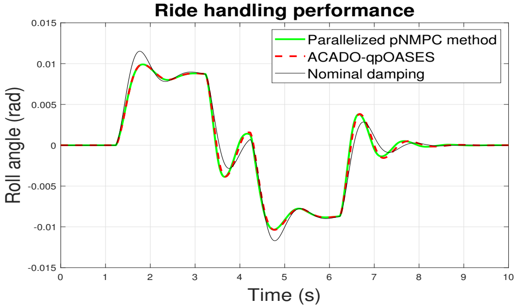
Figure 4.3: Ride handling - roll angle \theta
