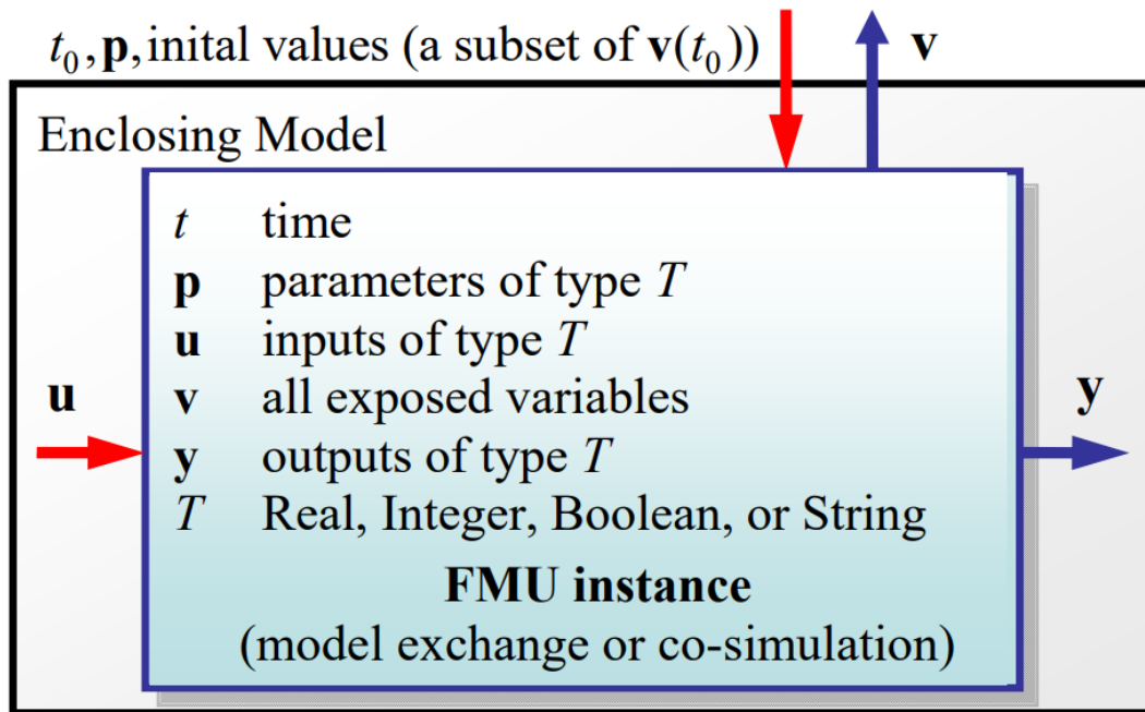
Figure 1.7: Schematic of data flow between the simulation tool and the FMU [Blockwitz et al. 2012]
