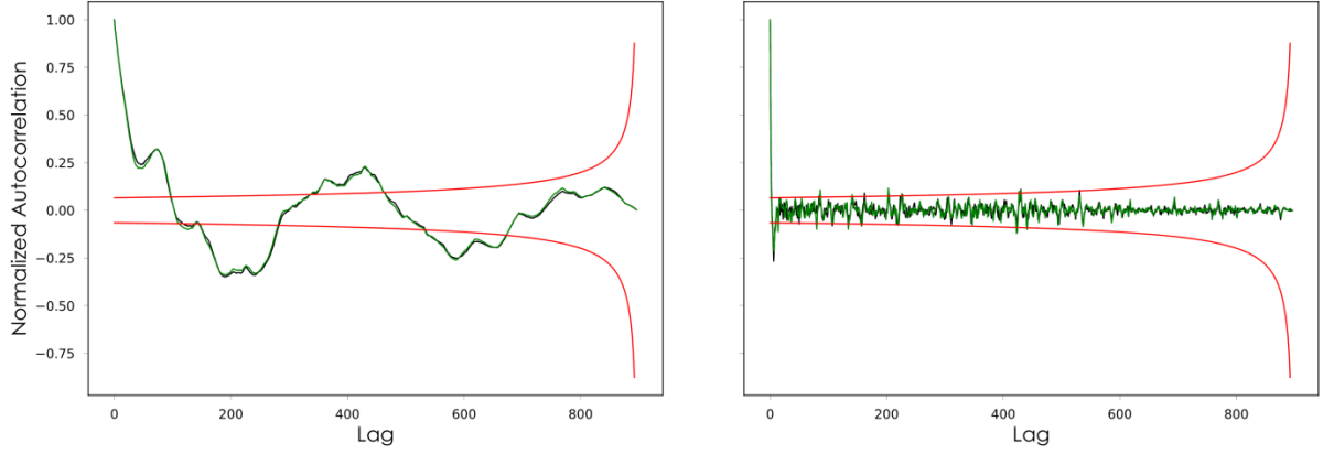
Fig. 54. Correlogram before ( left ) and after ( right ) applying the HPF; Alice and Bob's profiles are shown respectively in green and black, the NIST 95% confidence interval boundary in red
