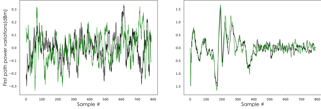
Fig. 53. Examples of FPP profiles obtained by the two parties in the worst ( left ) and best ( right ) configurations; the profiles have been centered on their mean
