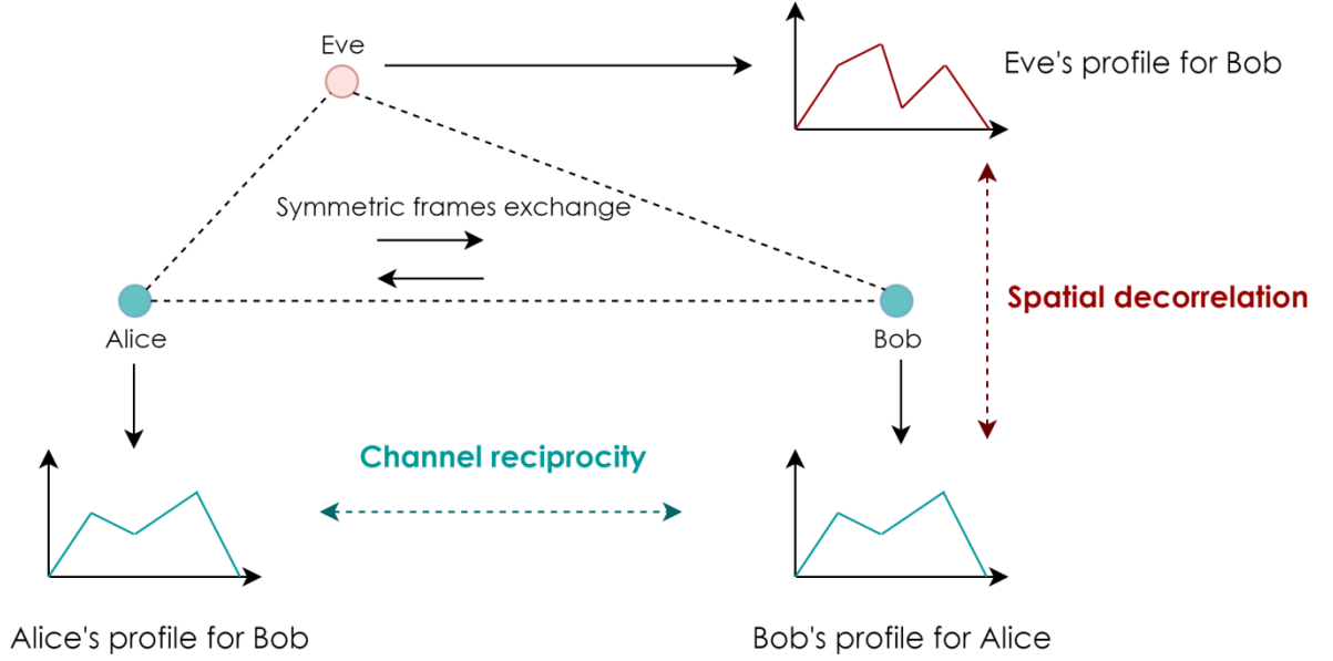
Fig. 52. Principles of Channel-based Key Extraction
