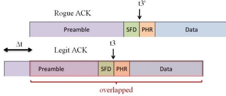
Fig. 23. Preamble overlap
