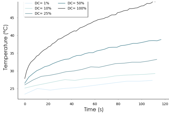
Fig. 48. For different duty cycles (DC) at Text = 23^{\circ}\text{C}
