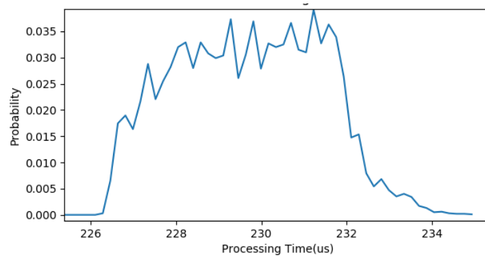
Fig. 22. \Delta t_{23} probability distribution (SPI speed = 20 Mhz, Preamble Length = 64 Symbols)
