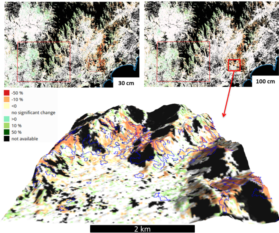
Figure 24 : Potential SOC change map 1991-2011 for the 0-30 cm and 0-100 cm soil layers and a 3D landscape view. The area in white represents no significant change and no data is available for the areas in black. The blue polyline encloses the areas subject to deforestation between 1990 and 2010 (MEFT, 2009; Grinand et al, 2013).
