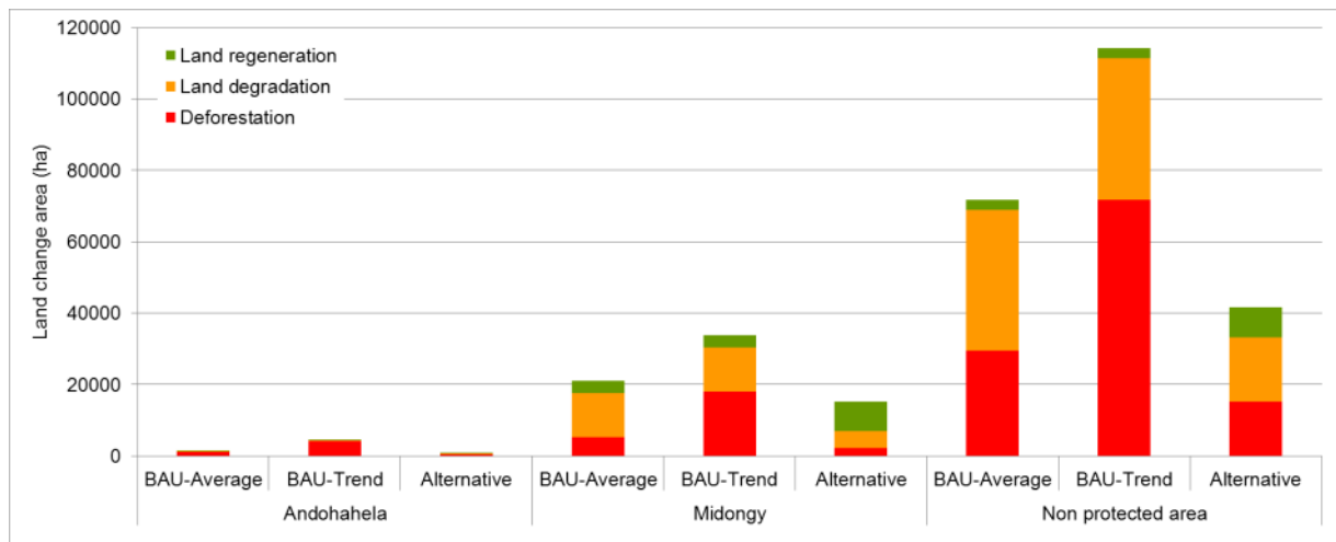
Figure 35 : Land change allocation results according to the three scenarios for different extents: the Andohela National Parks, the Midongy National Parks and outside those two perimeters.
