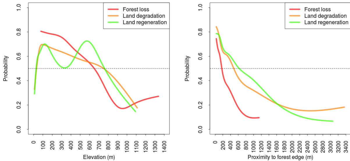
Figure 31 : Illustration of the two main predictors (elevation and distance to the forest edge) effects regarding deforestation, land degradation and land regeneration.
