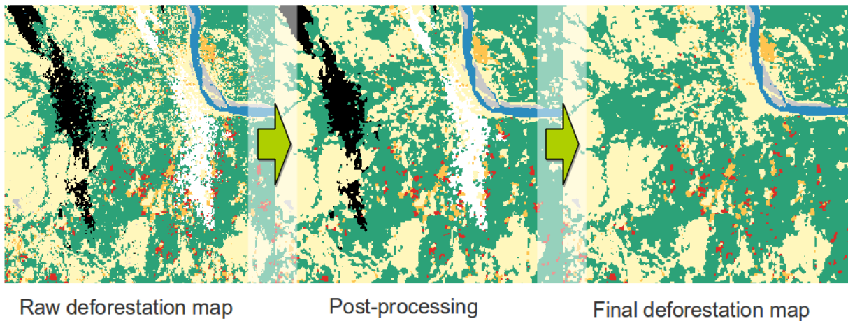
Figure 16 :Illustration of post-processing steps: 1) minimum mapping unit filtering of 0.36 ha using a 3x3 moving window that retains only 2x2 deforestation patches and applies a majority vote for other categories (first to second panel) and 2) cloud and shadow removal using the 2005 forest map (second to third panel). Green represents the extent of the forest, light yellow the non forest, orange deforestation in the 2000-2005 interval, and red deforestation in the 2005-2010 interval. White pixels represent clouds, and black pixels shadows.
