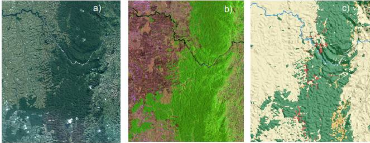
Figure 19 :Satellite images and final map of forest cover change for the periods 2000-2005-2010. a) QuickBird/Google Earth acquired on March 17, 2011. b) Landsat false colour composite RGB=TM5-3-2 acquired on November 17, 2010. c) Forest Cover Change 2000-2010 map, green represents the extent of the forest, light yellow represents non-forest, orange represents deforestation between 2000 and 2005, and red represents deforestation between 2005 and 2010. The FCC map is available in kmz format in supplementary material.
