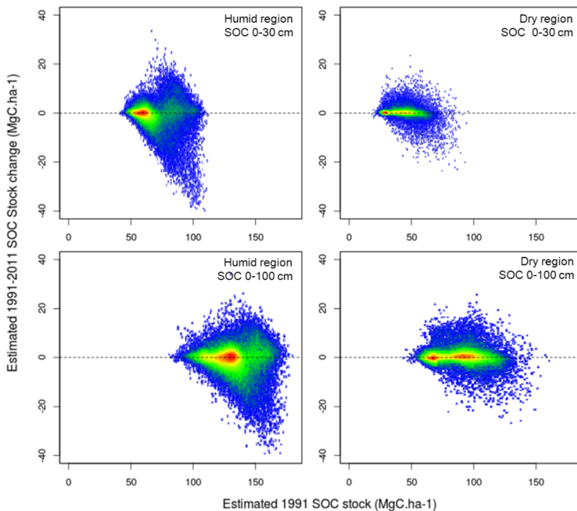
Figure 25 : Potential changes in SOC stocks estimated as a function of the initial stocks over the study area. Each graph were created using 100 000 observations/pixels randomly selected. Colors indicate density of observations/pixels (from white-blue to green, red).
