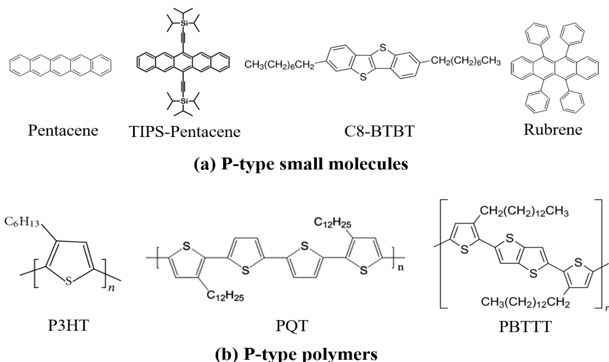
Figure 1.7 Molecular Structures of some typical P-type organic semiconductors with high mobility (a) small molecules, (b) polymers.
