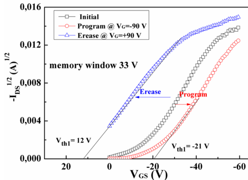
Figure 3.15 The typical memory transfer curves of SFG memory with PFBT monolayer, plotted with (I_{DS})^{1/2} versus V_{GS} after gate bias pulses \pm 90 \text{ V} for 10 s.
