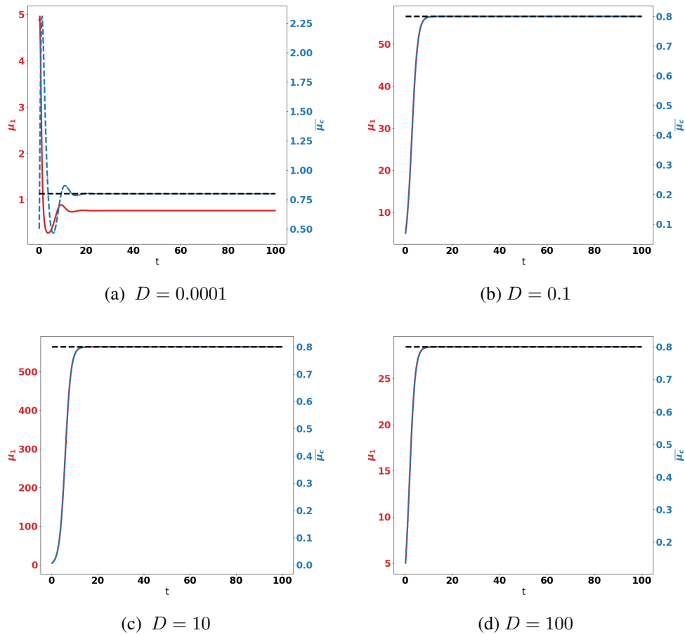
FIGURE 2.11 – Non saturated interactions, homogeneous source of immune cells. Evolution of the tumor mass \mu_1 (red curves, left axis), and of \bar{\mu}_c (blue curve, right axis) for several values of the diffusion coefficient D .
