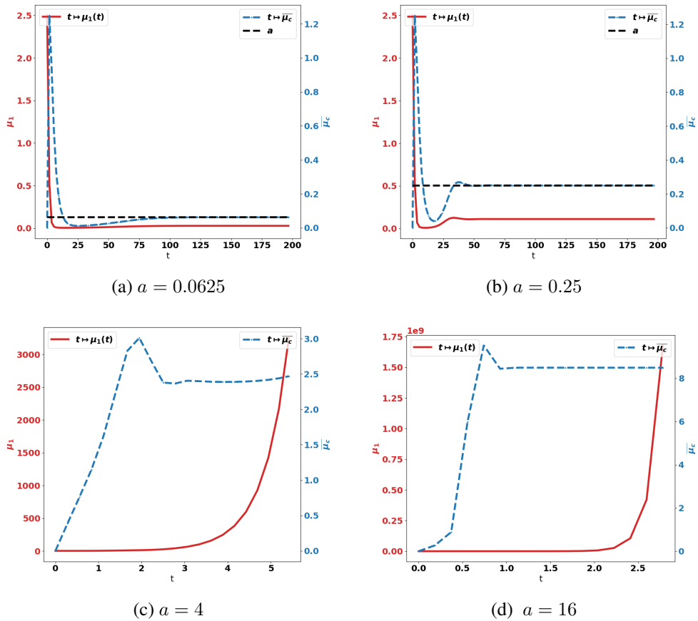
FIGURE 4.6 – Evolution of the tumor mass \mu_1 (red curves, left axis), and of the immune strength \bar{\mu}_c (blue curve, right axis) for several values of the division rate a
