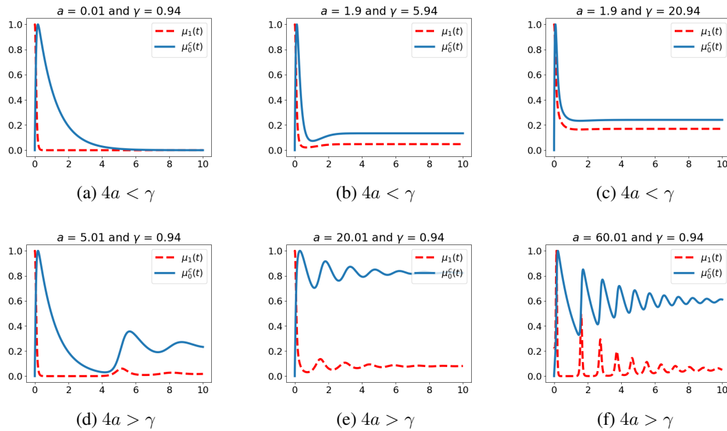
FIGURE 2.1 – Typical behavior of the solutions of (2.25). The data are : V = 0.616 , \delta = 0.5 , p = 4.66 , S = 6.38 (x-axis : time, y-axis : \mu_1 , mass of the tumor, and \mu_c , the total number of active immune cells).
