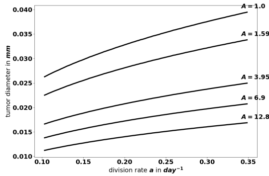
(a) different values for the pair (a, A)
