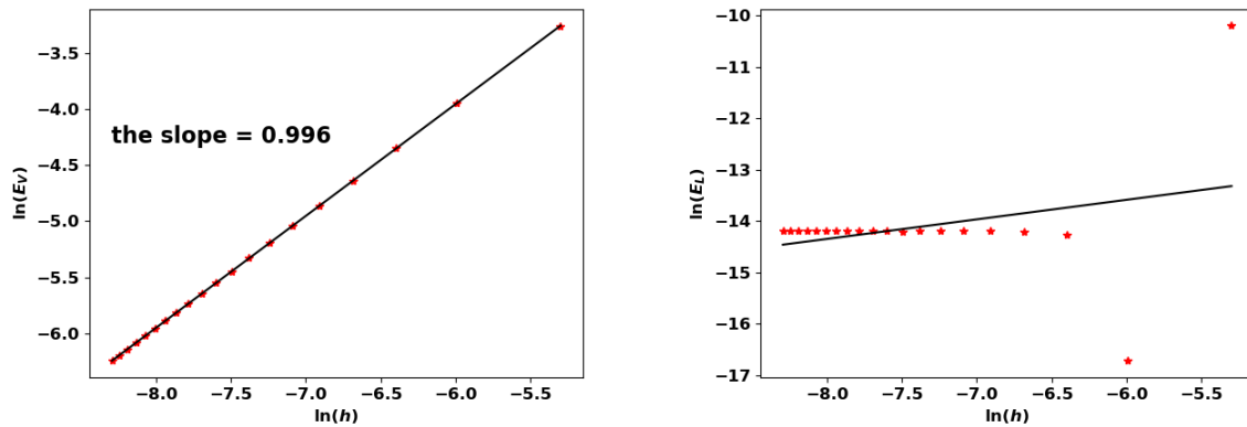
(a) The rate of convergence to the exact eigenfunction with respect to h
