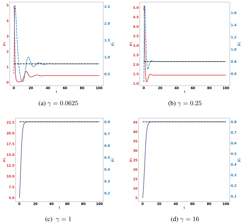
FIGURE 2.8 – Non saturated interactions, homogeneous source of immune cells. Evolution of the tumor mass \mu_1 (red curves, left axis), and of \bar{\mu}_c (blue curve, right axis) for several values of the immune cells death rate \gamma
