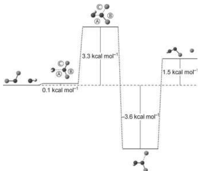
Figure 5. Calculated potential-energy surface for the \text{OH} + \text{Cl}_2\text{O} reaction leading to the formation of \text{HOCl} and \text{Cl} products. Energies were calculated at the UMPW1K/6-311++G(2df,p) level.
