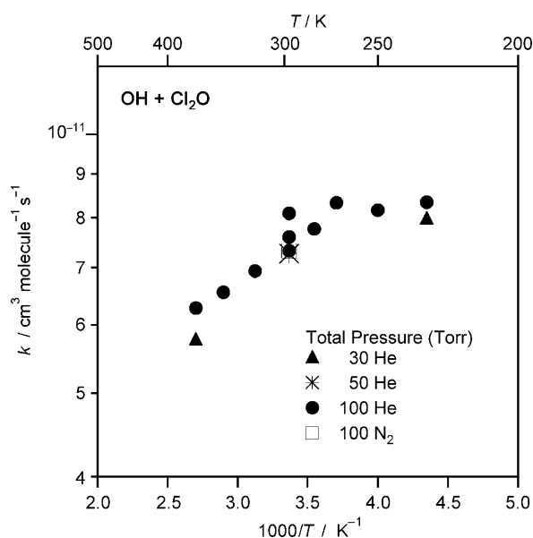
Figure 2. Temperature dependence of rate coefficient for the OH + \text{Cl}_2\text{O} reaction obtained in this work. The symbol size represents the 2\sigma uncertainty from the precision of the measurement.
