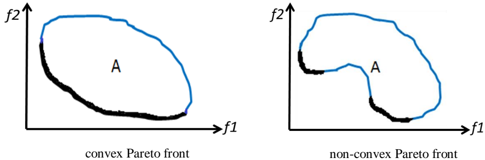
Figure 2.2 Pareto front for a bi-objective problem
