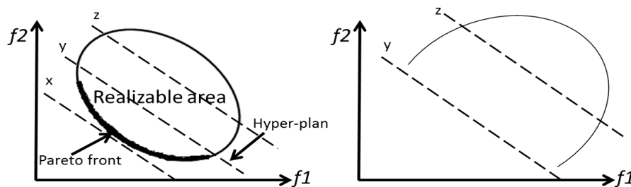
Figure 2.3 Pareto Solutions
