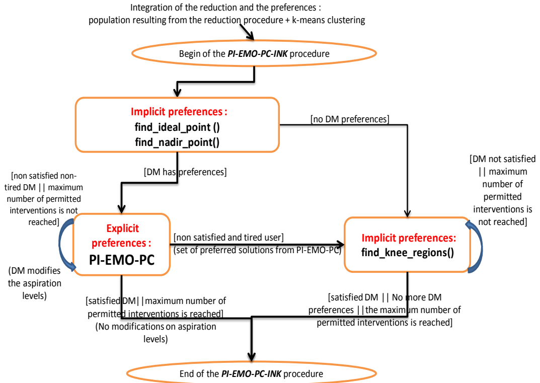
Figure 3.6 The proposed hybrid preference algorithm (PI-EMO-PC-INK)
