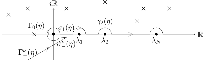
Figure 3.1: The curve \Gamma^\nu(\eta) . \lambda_1, \dots, \lambda_N are the outgoing positive resonances of H .
