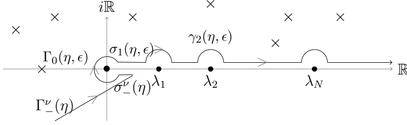
Figure 3.2: The curve \Gamma^\nu(\eta, \epsilon) .
