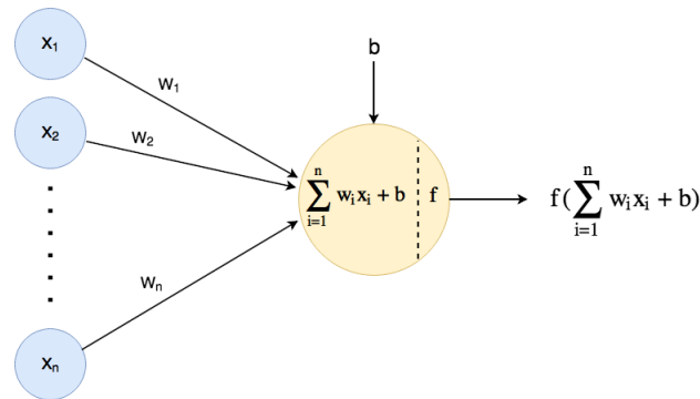
Figure 4.1 – Neuron
