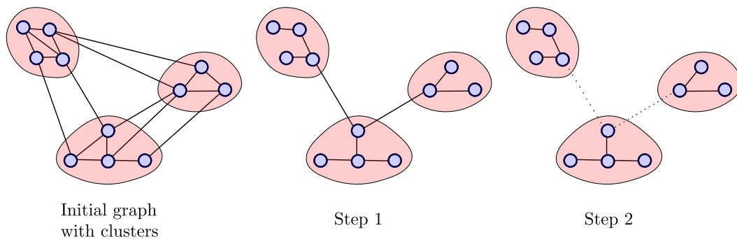
Figure B.1: Summary of the generic procedure for computing an MST-based clustering.
