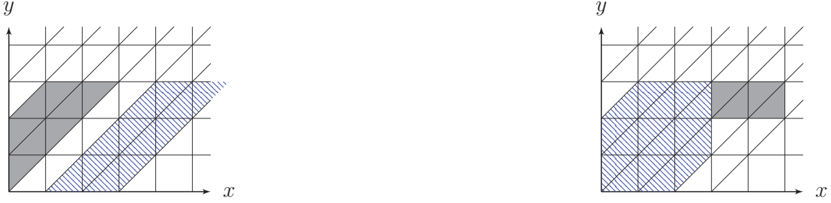
Figure 1.7 – For e = (\ell, g, a, R, \ell') with \text{Inv}(\ell) = \text{Inv}(\ell') = x \leq 6 \wedge y \leq 3 , g = x \geq 1 \wedge y \geq 1 and R = \{y\} , left figure represents in blue the successor of the gray zone by \text{Post}_e . On the right, the blue zone is the predecessor of the gray zone by \text{Pre}_e .
